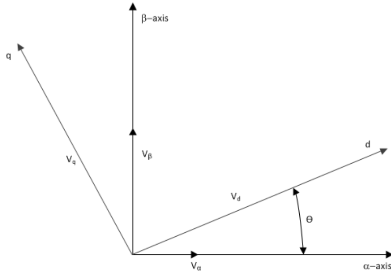
Figure 6 • Inverse Clarke Transformation
