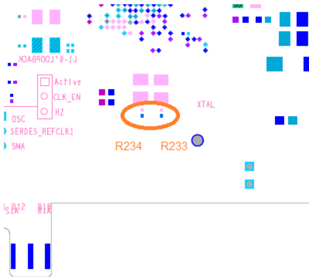
Figure 9 • Bottom Side Location of Series Resistors for SERDES_VDDAPLL Power Supply (R233 and R234)
