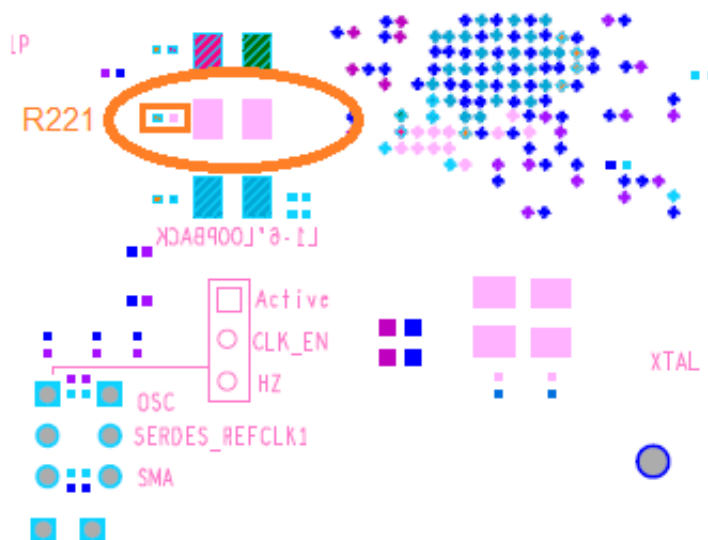
Figure 11 • Bottom Side Location of Series Resistor for SPLL Power Supply (R221)
