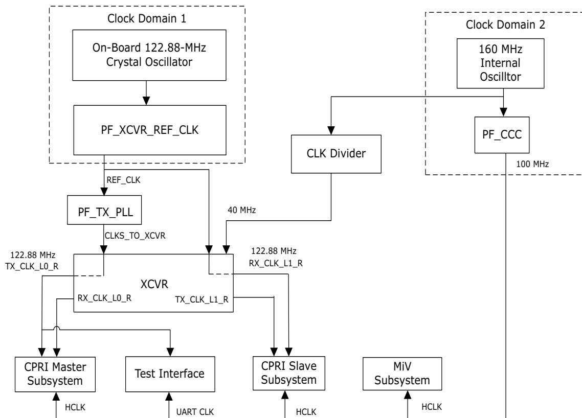
Figure 12 • Clocking Structure
