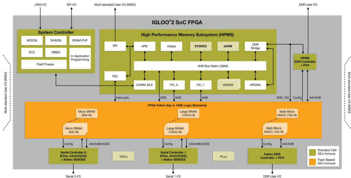
Figure 2 • IGLOO2 Architectural Block Diagram
