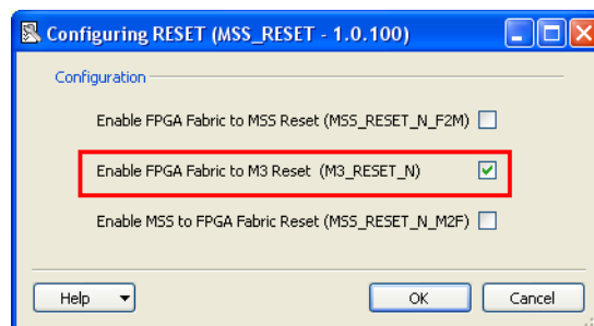
Figure 12 • Exposing M3_RESET_N to FPGA Fabric
