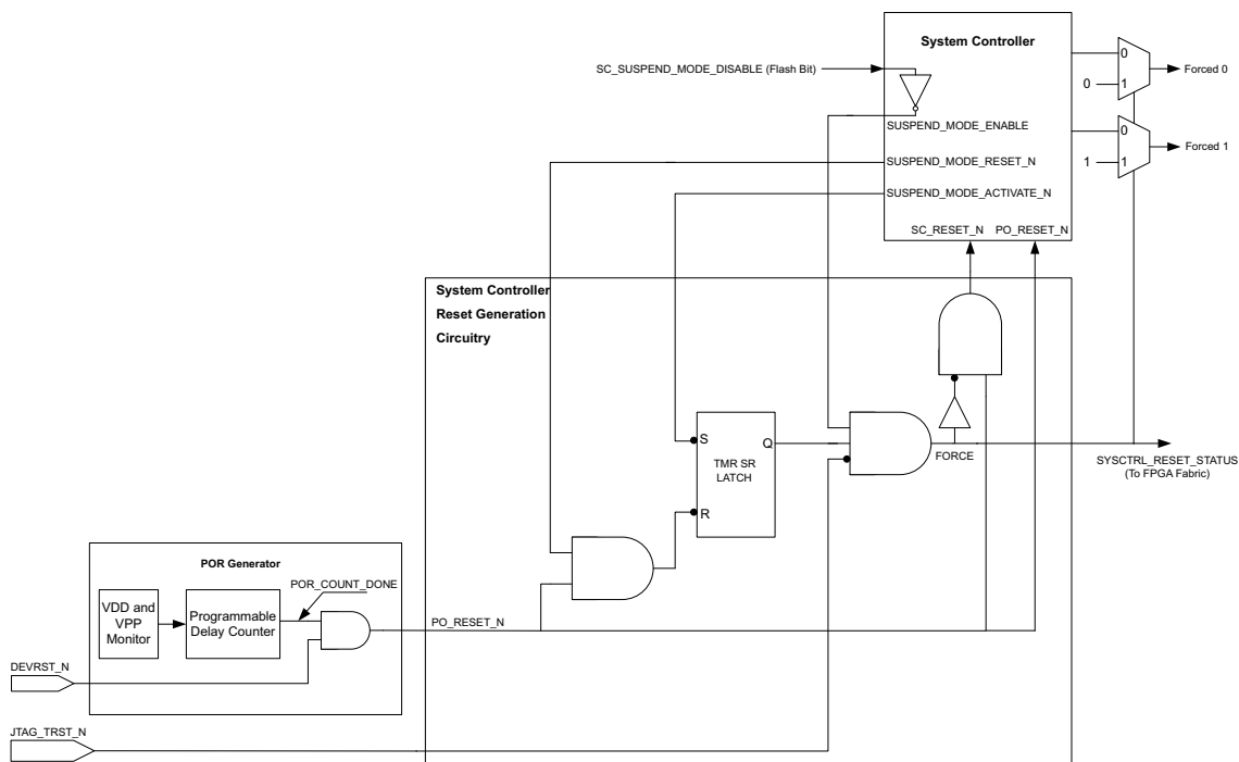
Figure 16 • System Controller Reset Generation Circuitry
