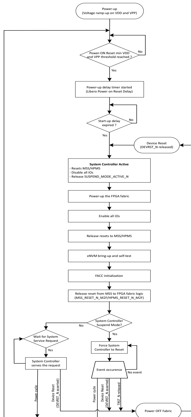
Figure 15 • Device Initialization Sequence Performed by System Controller
