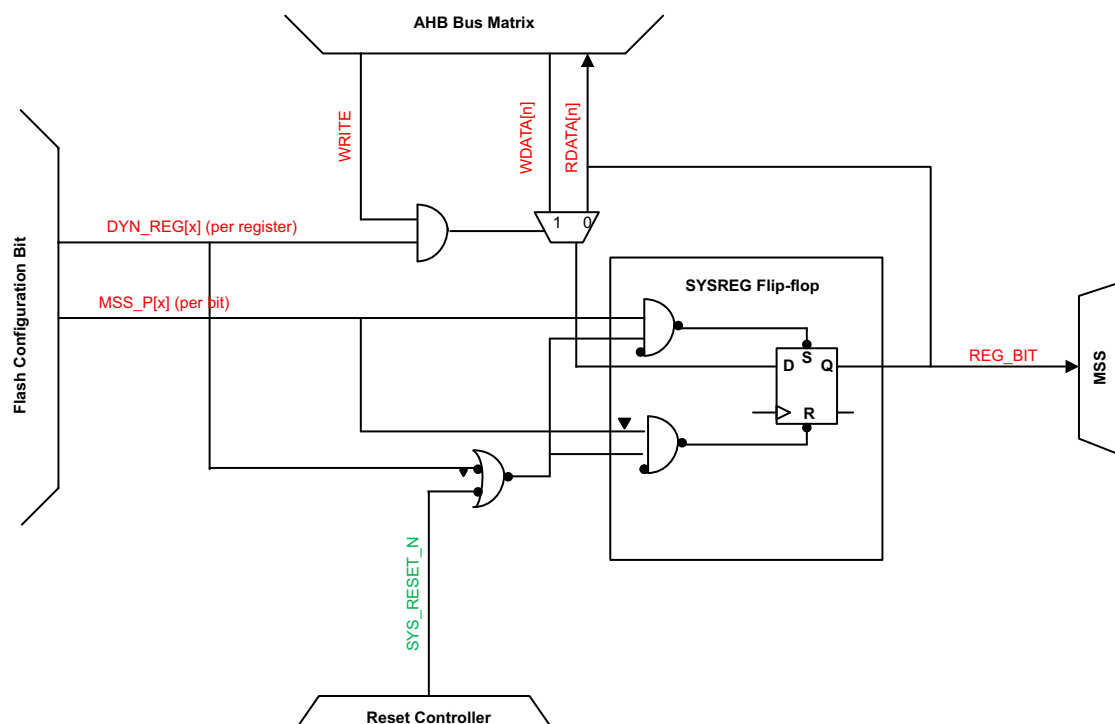
Figure 4 • System Register Schematic
