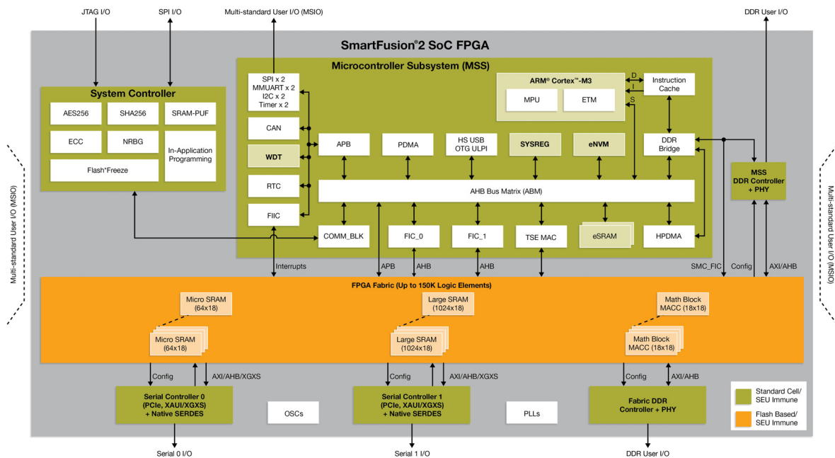
Figure 1 • SmartFusion2 Architectural Block Diagram
