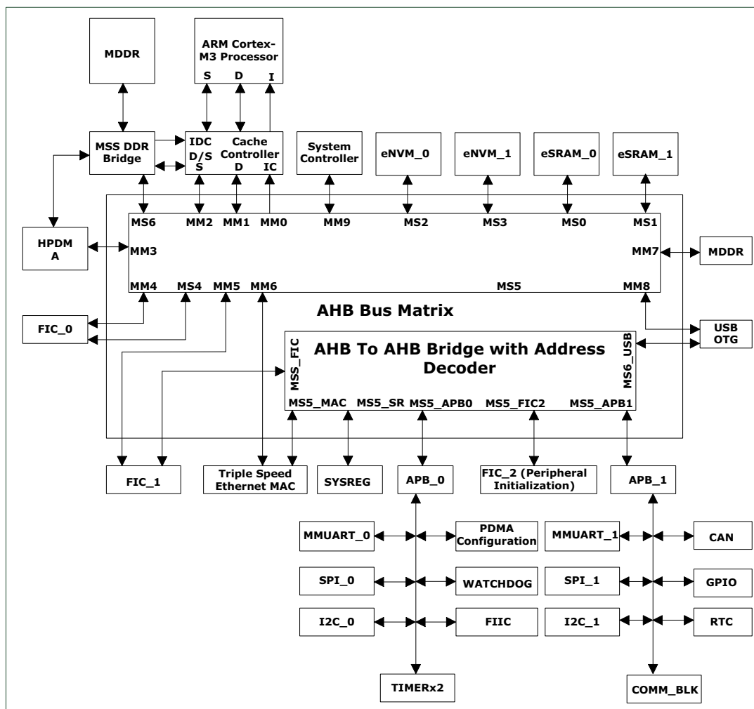
Figure 3 • SmartFusion2 MSS Block Diagram
