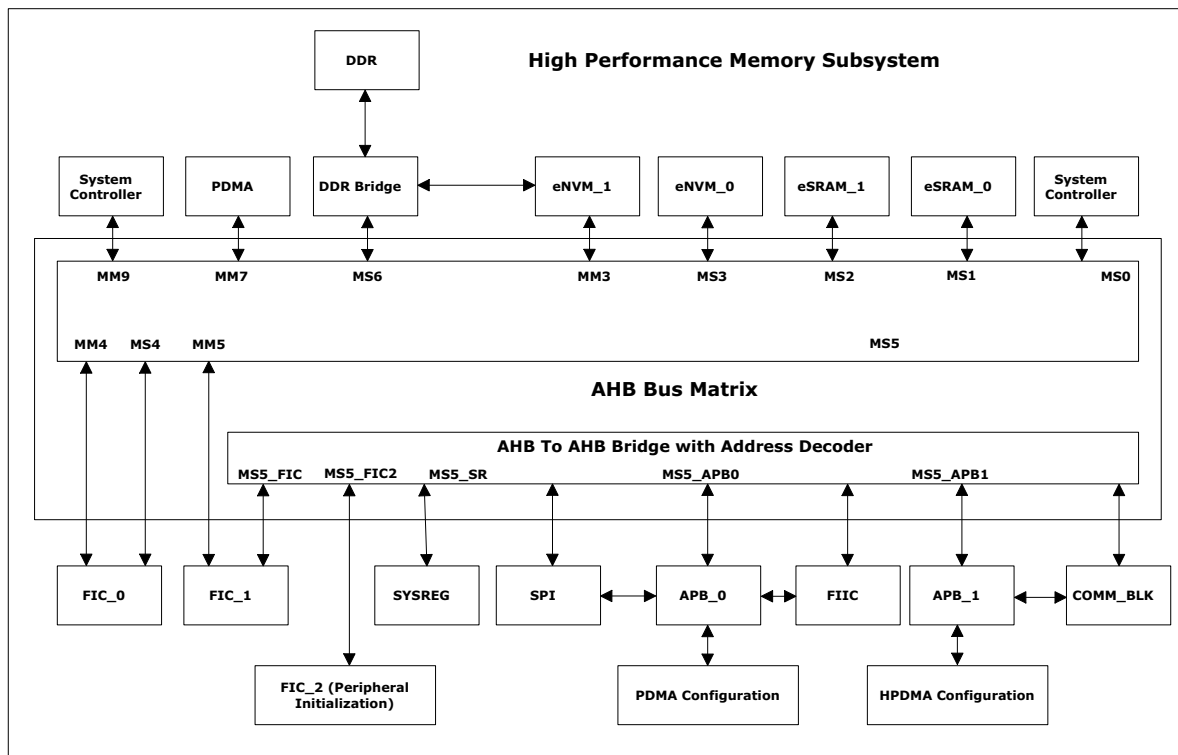
Figure 5 • IGLOO2 HPMS Block Diagram
