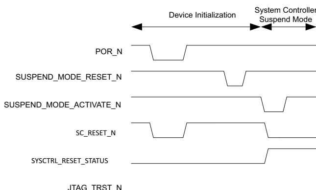
Figure 17 • System Controller Suspend Mode Activation after Device Initialization
