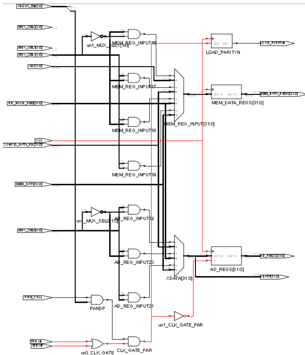
Figure 2 • Datapath Block Showing Critical Path for clk-out and External Setup
