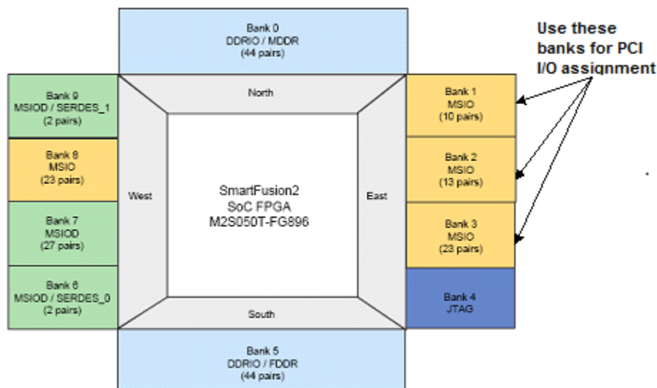
Figure 3 • PCI I/O Assignment in M2S050T Device for 33 MHz PCI Design
