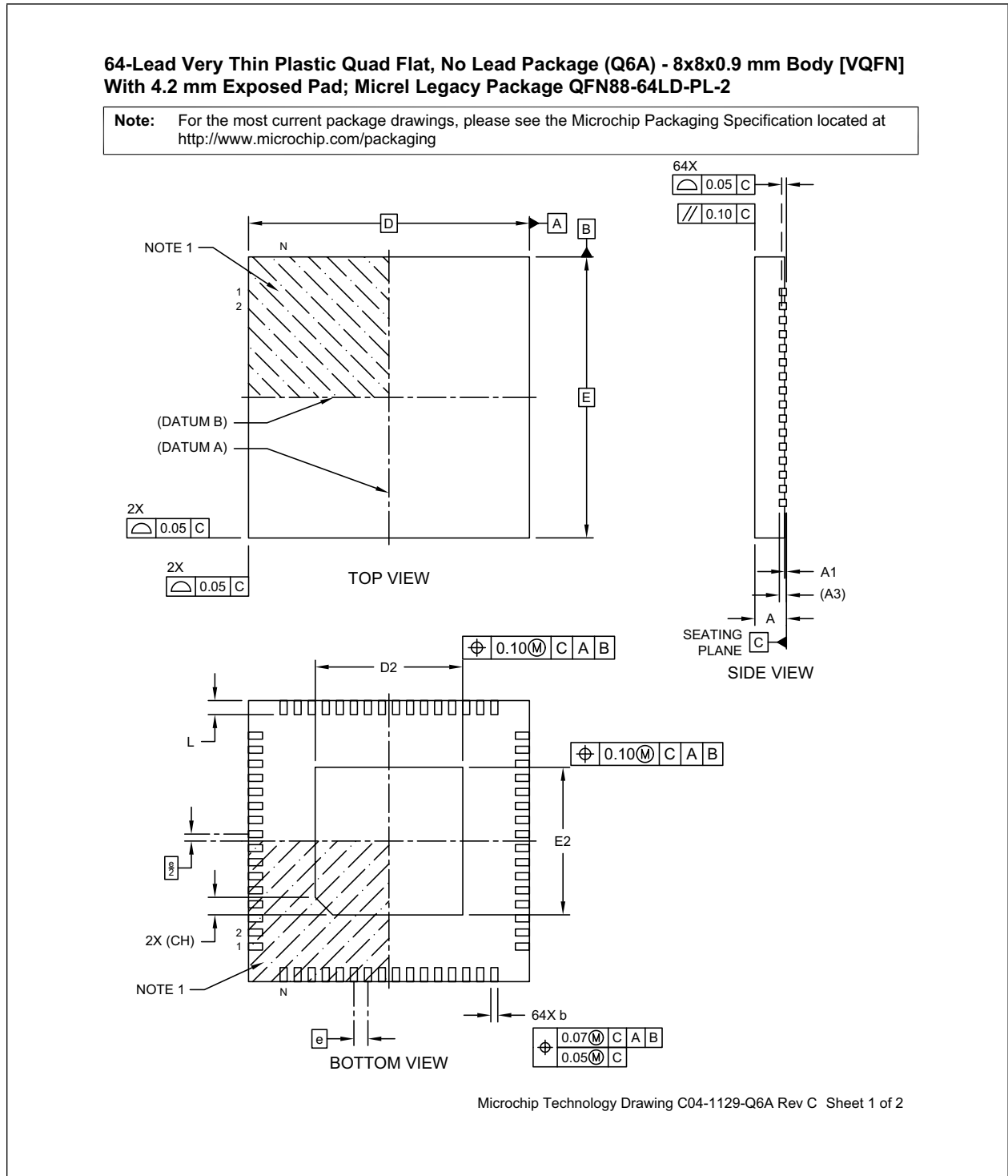
FIGURE 13-1: 64-VQFN PACKAGE WITH 4.2 MM EXPOSED PAD - DRAWING
