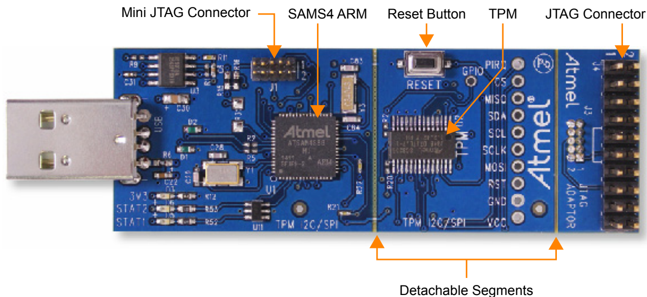
Figure 1. Atmel I 2 C/SPI Demonstration Kit
