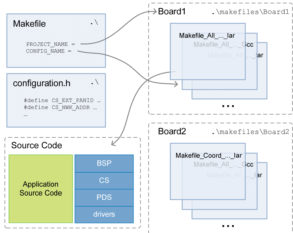
Figure 1-2. Application build structure with makefiles.
