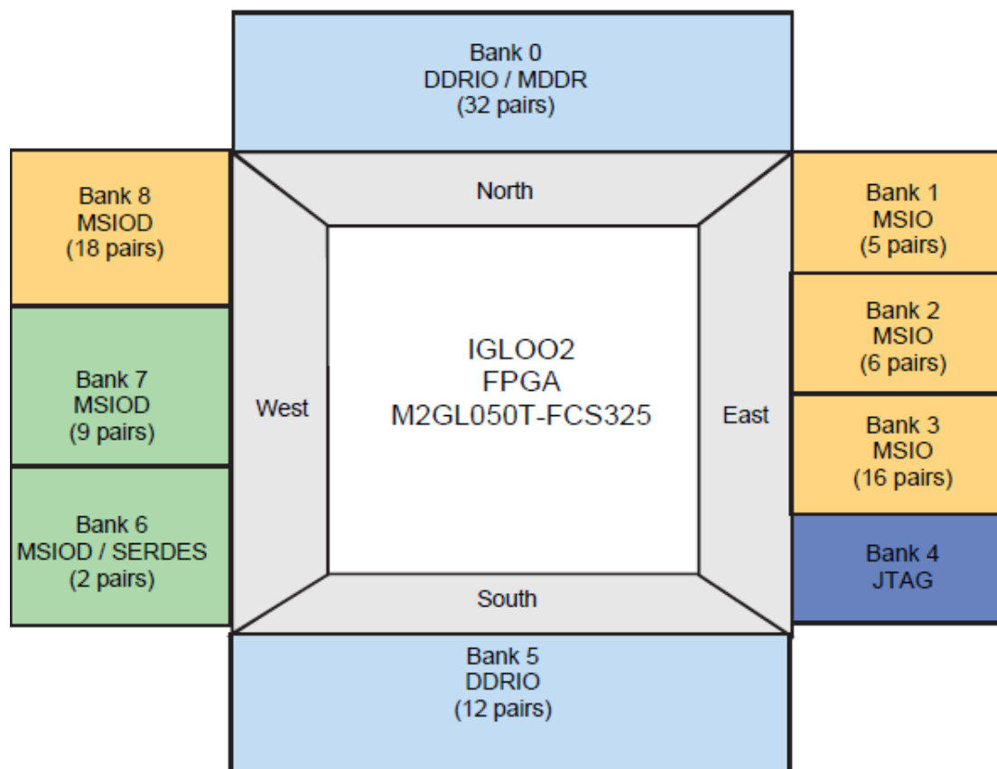
Figure 1 • IGLOO2 FPGA M2GL050T FCS325 I/O Bank Locations
