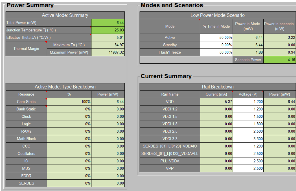
Figure 21 • Power Summary
