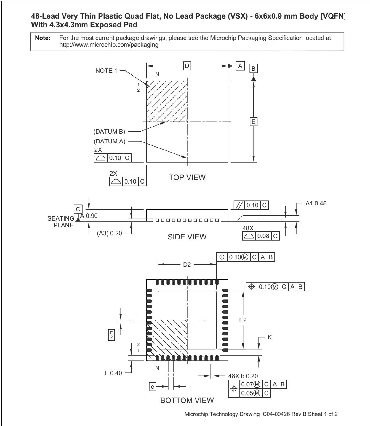
FIGURE 17-1: 48-LEAD QFN PACKAGE 6X6 MM (DRAWING)
