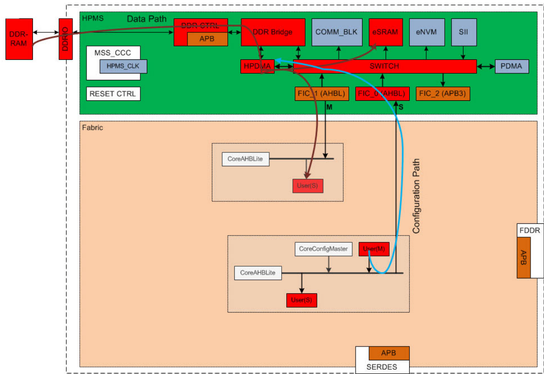
Figure 2 • User Fabric Master Configuring HPDMA to Initiate Transfers between HPMS DDR, eSRAM and User Fabric Slave
