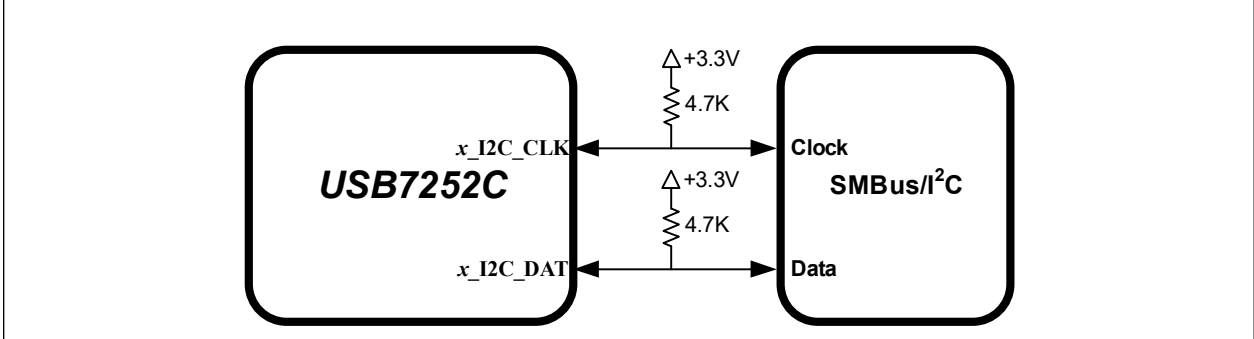
FIGURE 4-3: SMBUS/I 2 C CONNECTIONS
