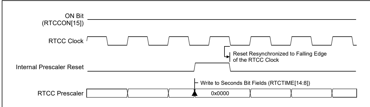
Figure 29-6: Prescaler Synchronization to Seconds Register Write
