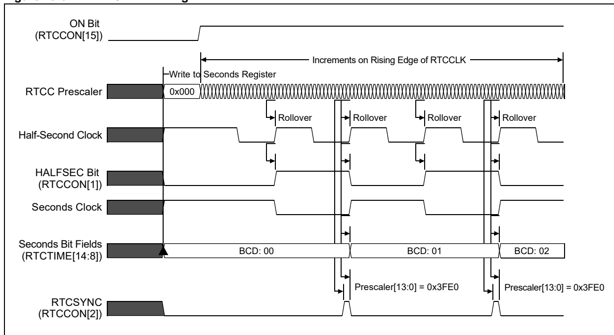
Figure 29-5: RTCSYNC Timing
