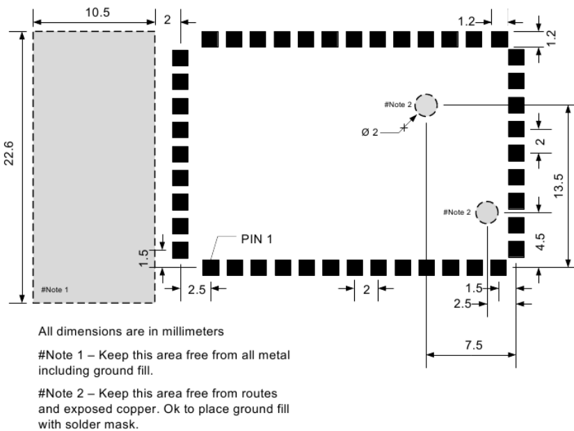
Figure 5. Pad Dimensions
