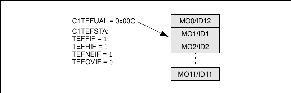
Figure 10-26: TEF – Full
