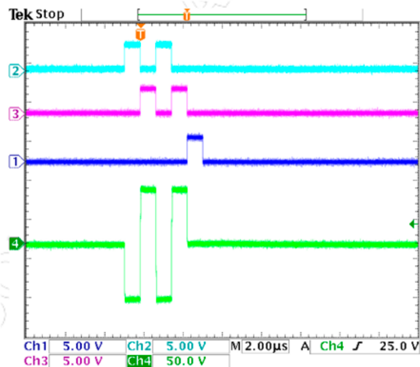
Fig 2: Input and output waveforms at V_{DD} = 10V , V_{PP}/V_{NN} = \pm 70V , Load = 330pF//2.5k.
