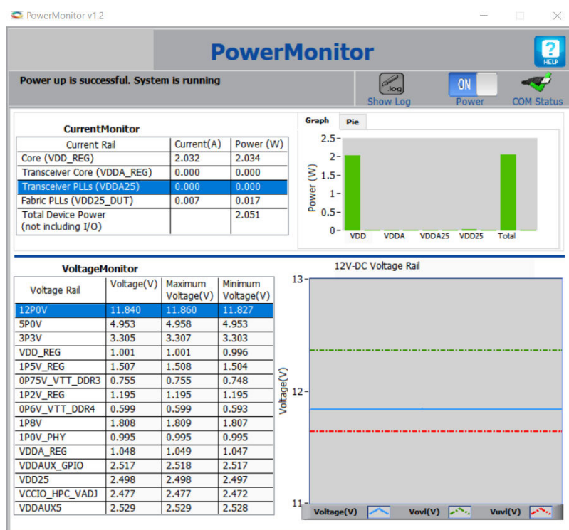
Figure 2-4. Total Power—XCVR and TX PLL
