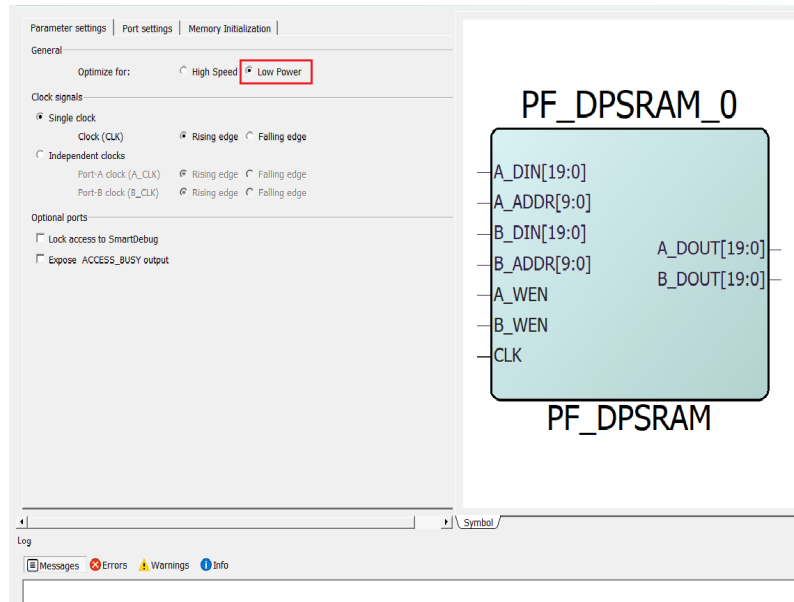
Figure 1-2. Low-Power Setting for Dual-Port LSRAM
