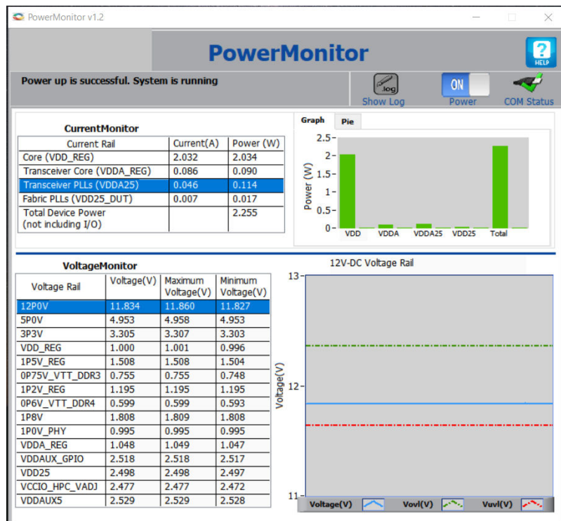
Figure 2-3. Total Power—PolarFire Low-Power Demo
