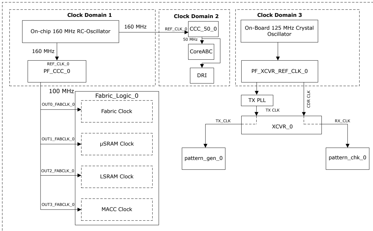
Figure 1-12. Clocking Structure
