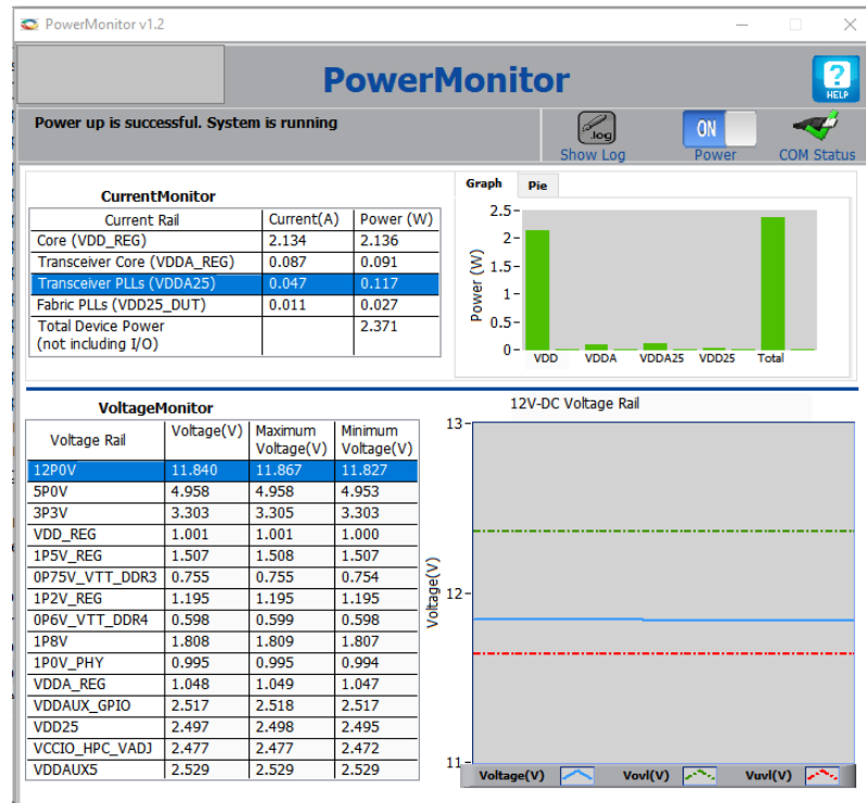
Figure 2-2. Total Power—PolarFire Normal Demo
