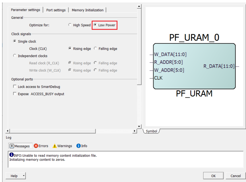
Figure 1-4. Low-Power Setting for Micro-SRAM
