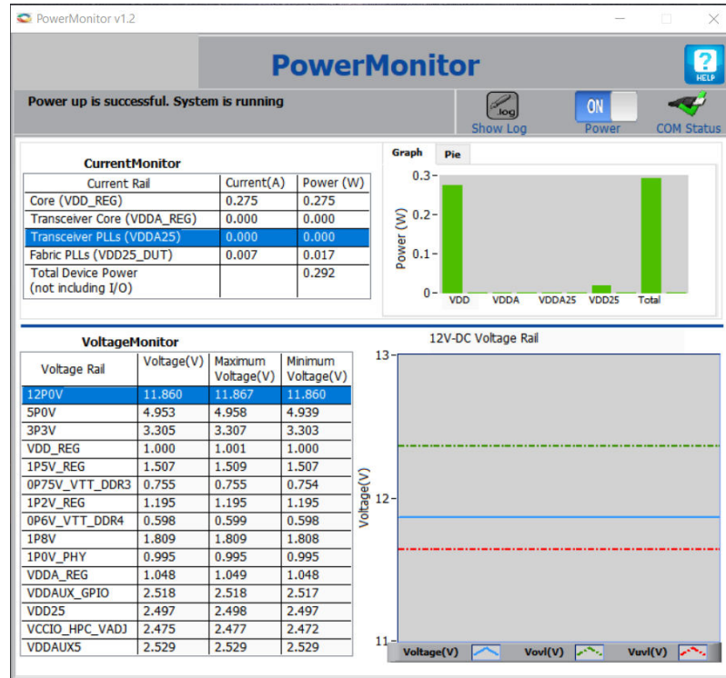
Figure 2-6. Total Power—Power Down Mode
