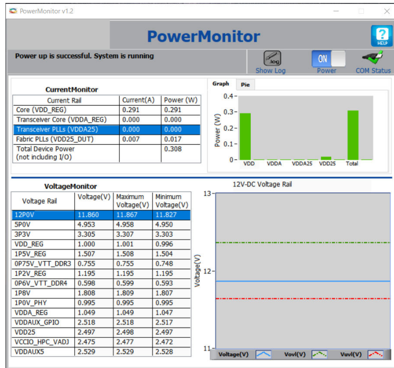
Figure 2-5. Total Power—Clock Gating
