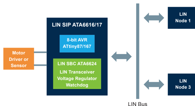
Figure 1. The ATA6616/17 LIN System-in-Package
