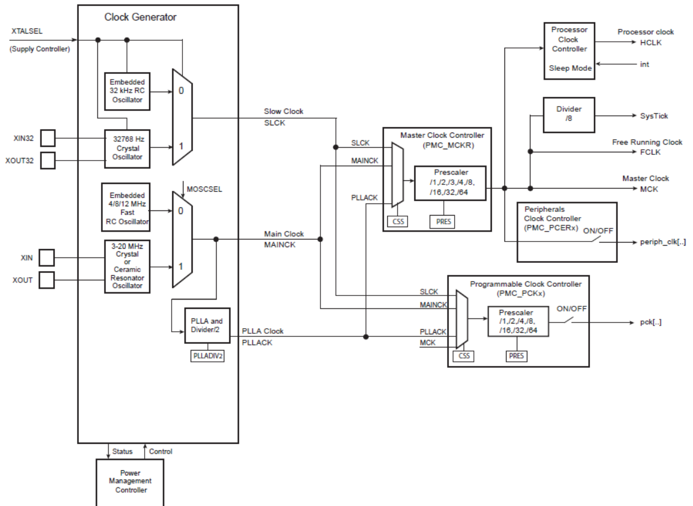
Figure 2-2. General Clock Block Diagram of SAM4N
