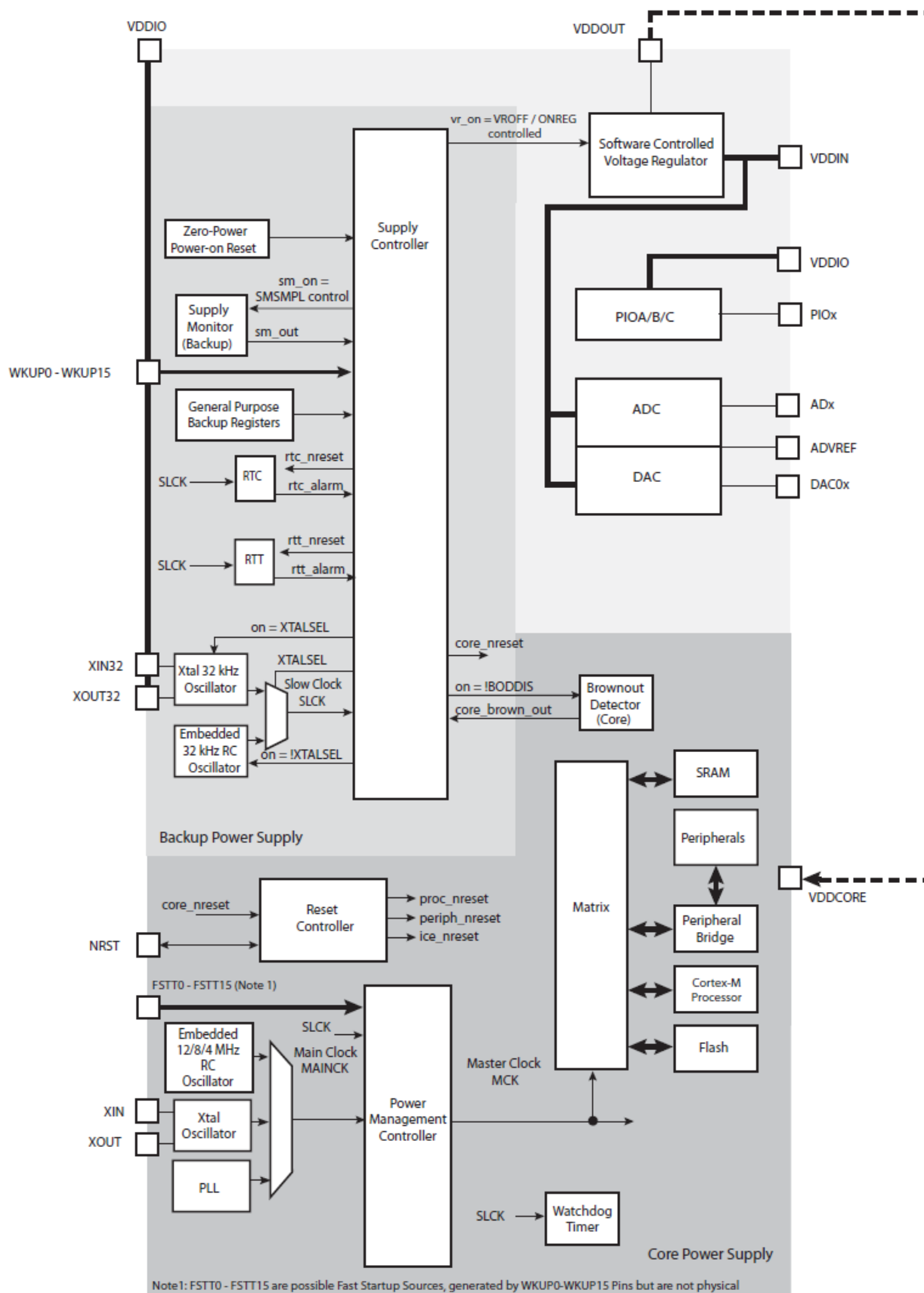
Figure 2-1. Supply Controller of SAM4N
