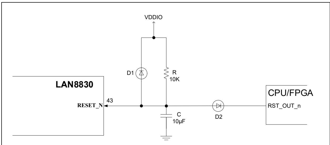
FIGURE 7-2: RESET CIRCUIT INTERFACE WITH CPU/FPGA RESET OUTPUT
