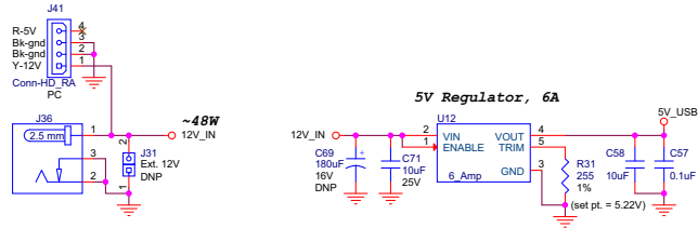
FIGURE B-2: EVB-USB4624BCUH EVALUATION BOARD SCHEMATIC 2
