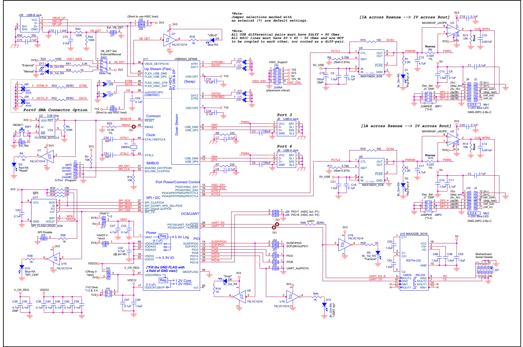
FIGURE B-1: EVB-USB4624BCUH EVALUATION BOARD SCHEMATIC 1
