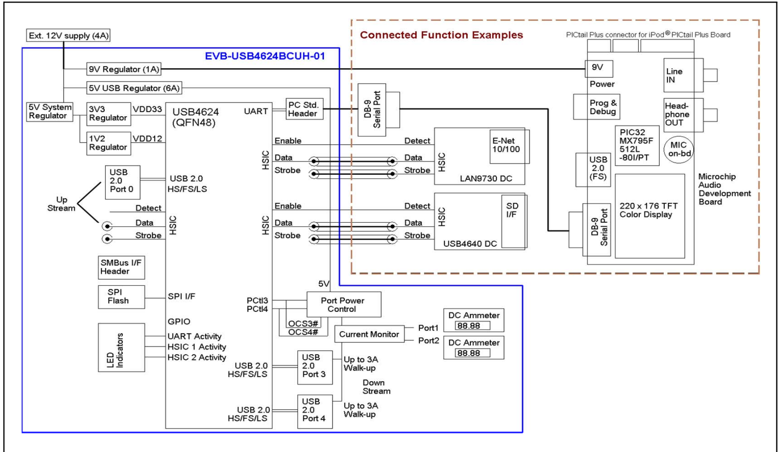
FIGURE 1-2: EVB-USB4624BCUH FUNCTIONAL BLOCK DIAGRAM
