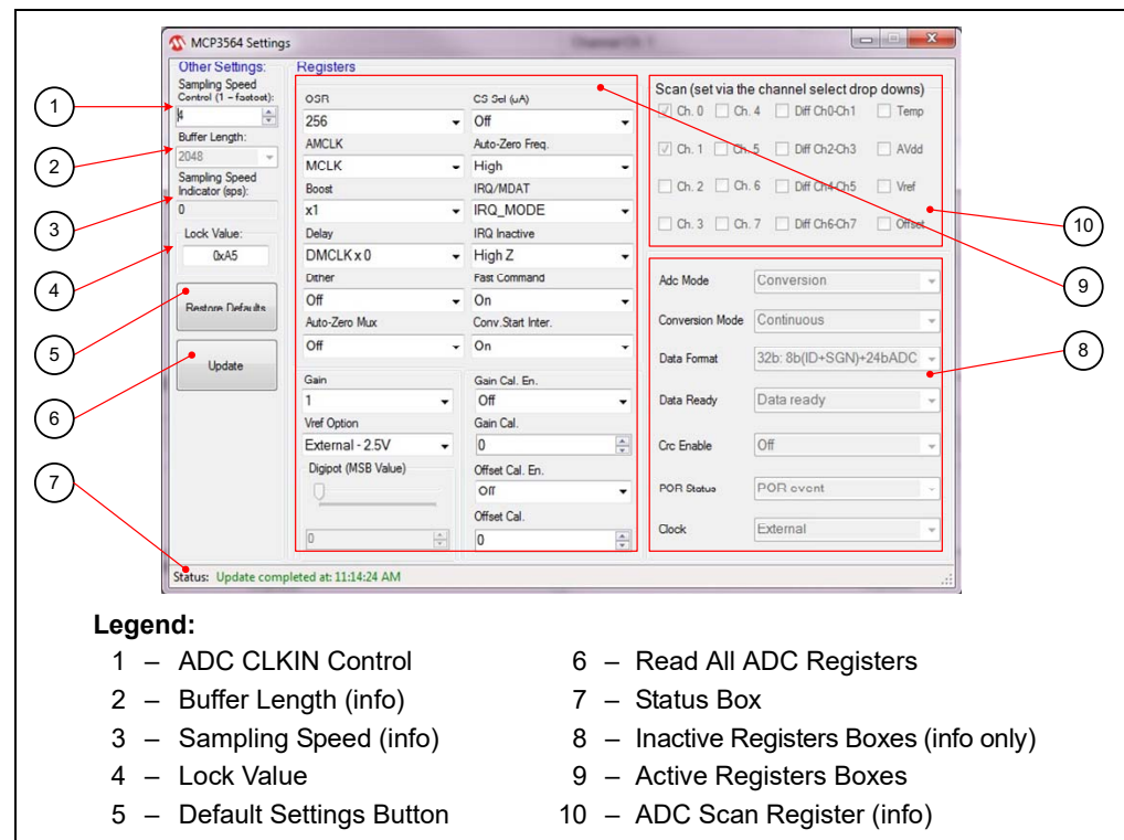
FIGURE 4-7: MCP3564 Settings Window.
