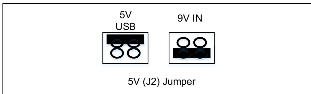
FIGURE 2-1: Power Source Selection.
