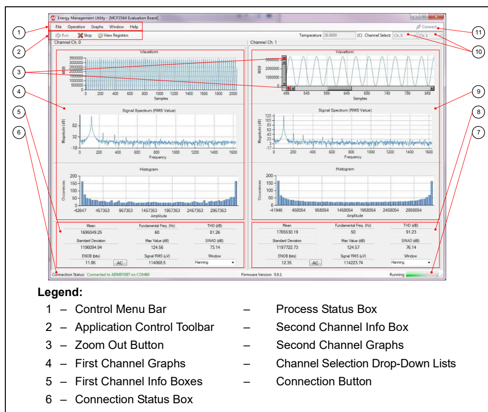
FIGURE 4-5: Main Window.
