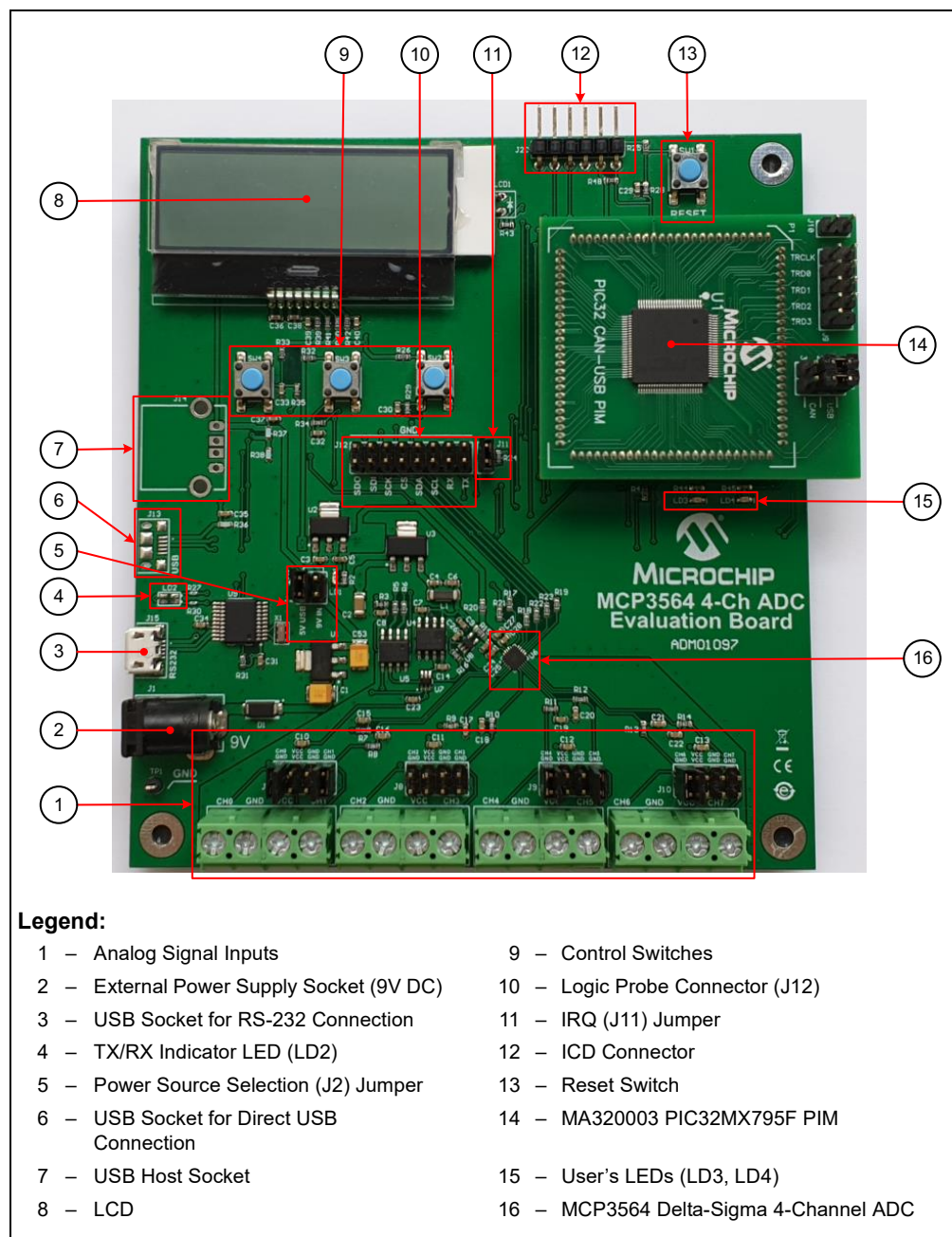
FIGURE 2-2: MCP3564 ADC Evaluation Board V2 Top View.
