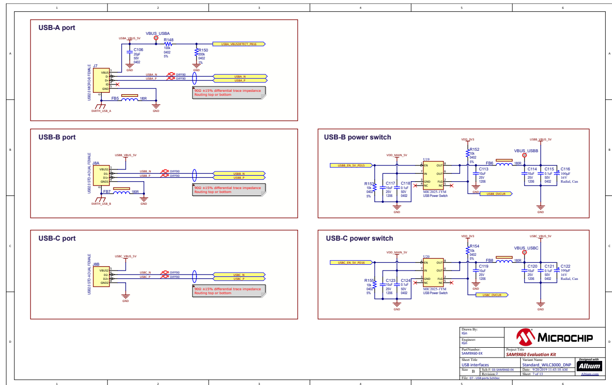
Figure 6-7. USB Interfaces
