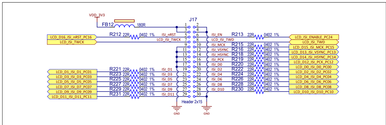
Figure 3-36. ISI Expansion Header
