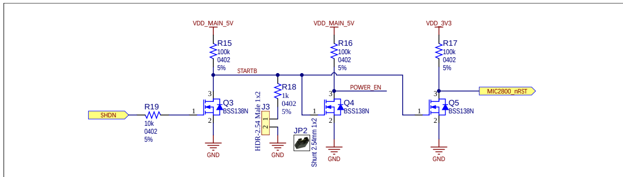
Figure 3-4. Shutdown Circuitry
