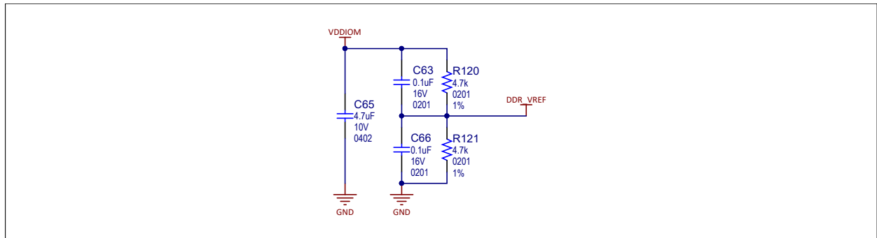
Figure 3-13. DDR Reference Voltage
