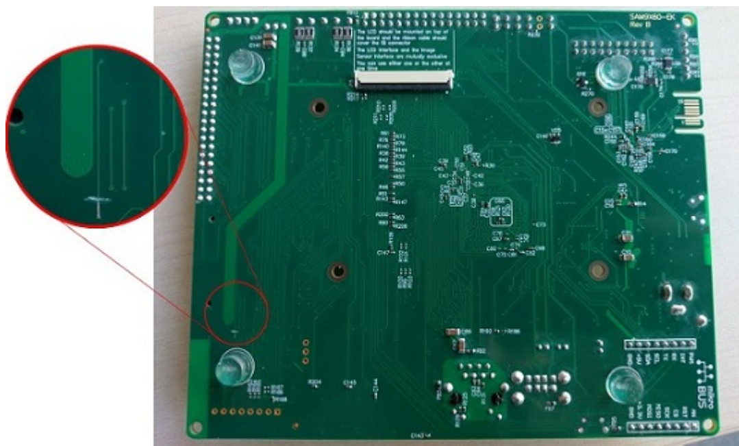
Figure 5-3. Board Modification Step 2
