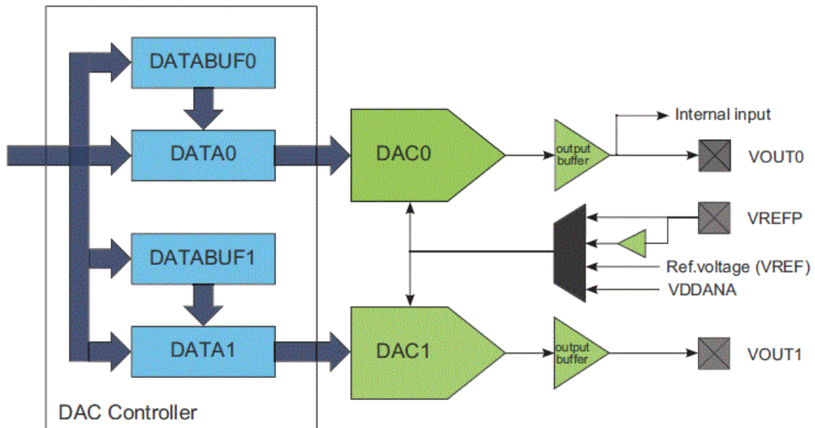
Figure 3-1 DAC Block Diagram
