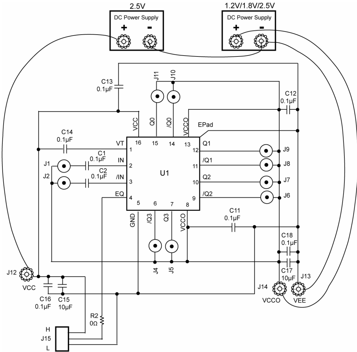
SY56020R AC-Coupled Evaluation Board
