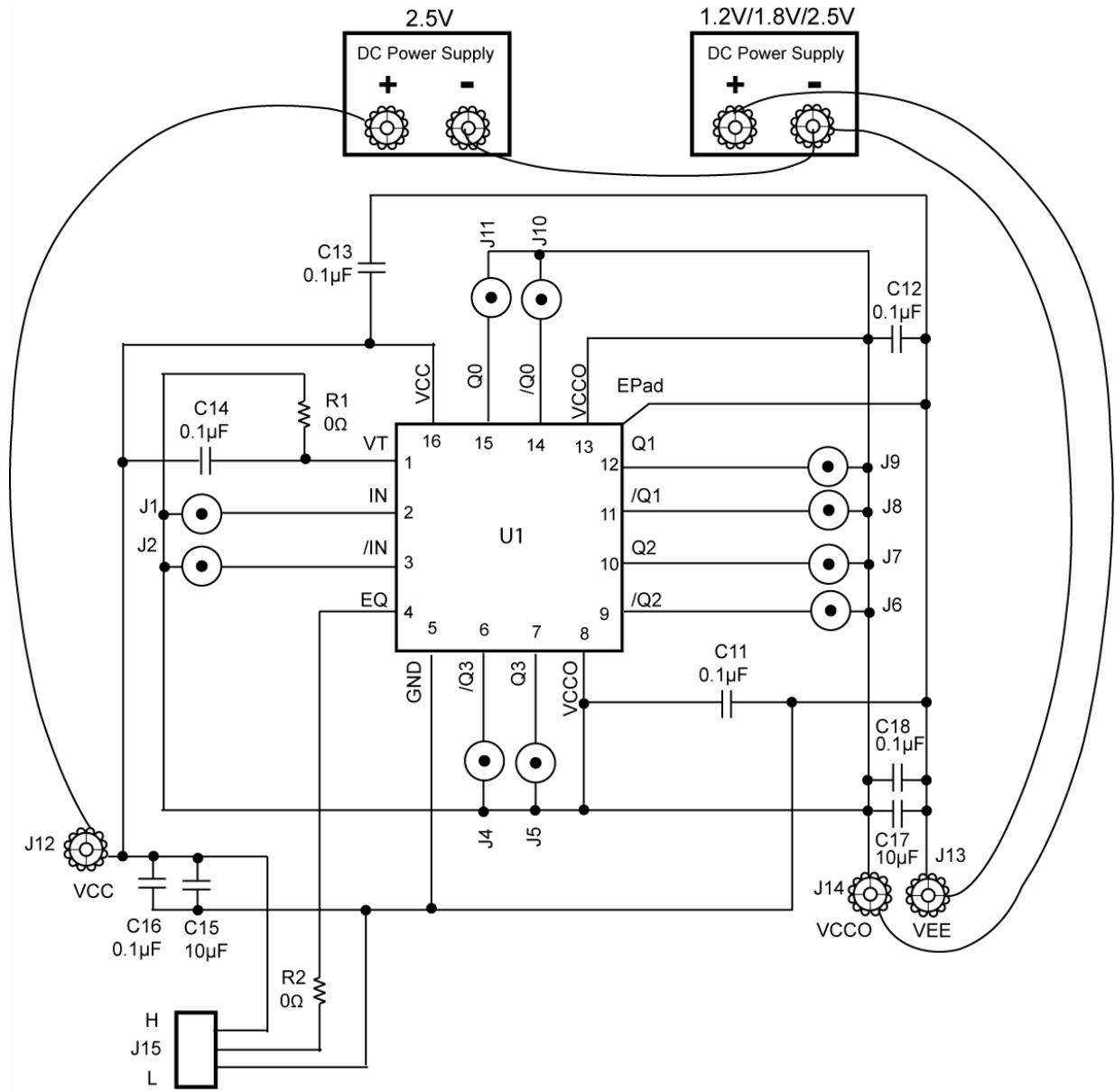
SY56020R DC-Coupled Evaluation Board
