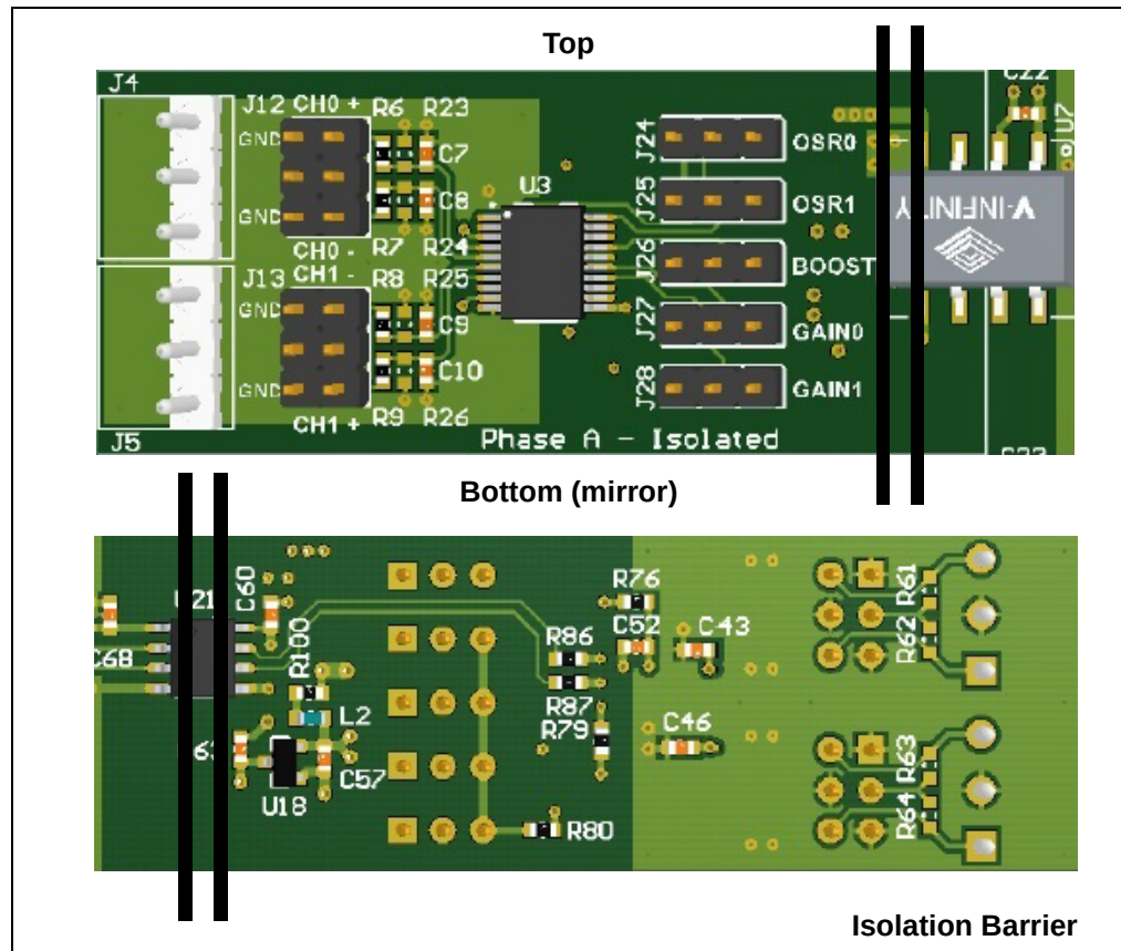
FIGURE 1-8: Isolated MCP3910(A), MCP3910(B), and MCP3910(C) Description.
