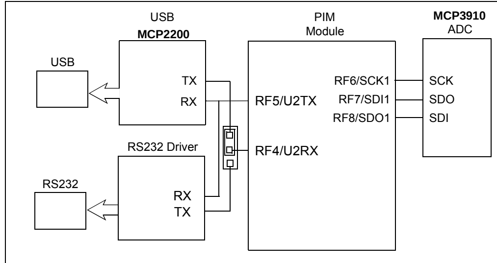
FIGURE 1-10: USB Block Diagram.
