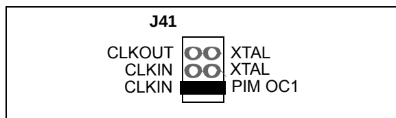
FIGURE 1-6: MCP3910(N) Clock Selection Jumpers - Clock from MCU.
