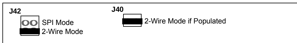
FIGURE 1-7: Selecting the MCP3910(N) to be Used in 2-Wire Mode.
