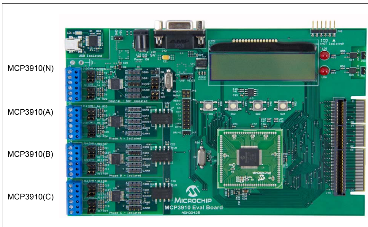
FIGURE 1-2: MCP3910 Evaluation Board.
