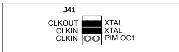
FIGURE 1-5: MCP3910(N) Clock Selection Jumpers - External Crystal.
