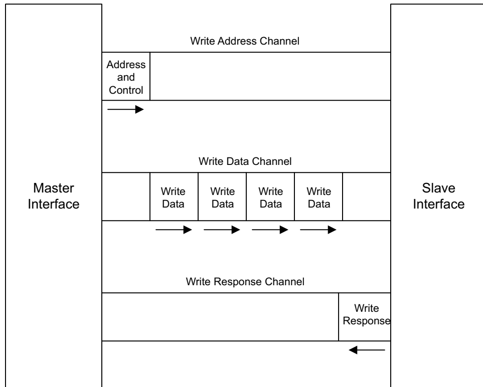
Figure 1 • AXI Write Flow
