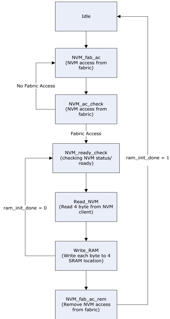
Figure 3 • Fabric Master State Diagram
