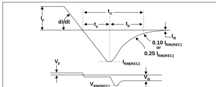
Figure 1. Typical Rectifier Response for Reverse Recovery
