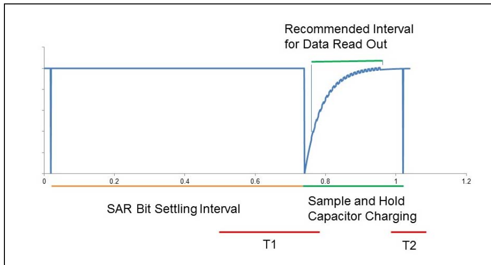
FIGURE 3-2: Recommended Period for Data Read Out.
