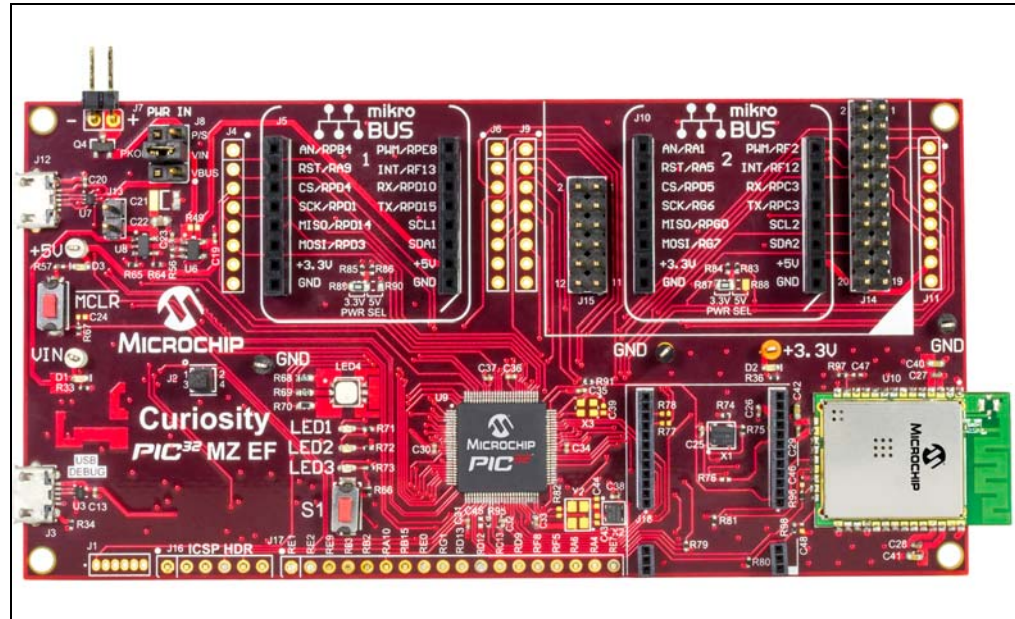
FIGURE 1-4: Curiosity PIC32MZEZ Development Board (DM320104).
