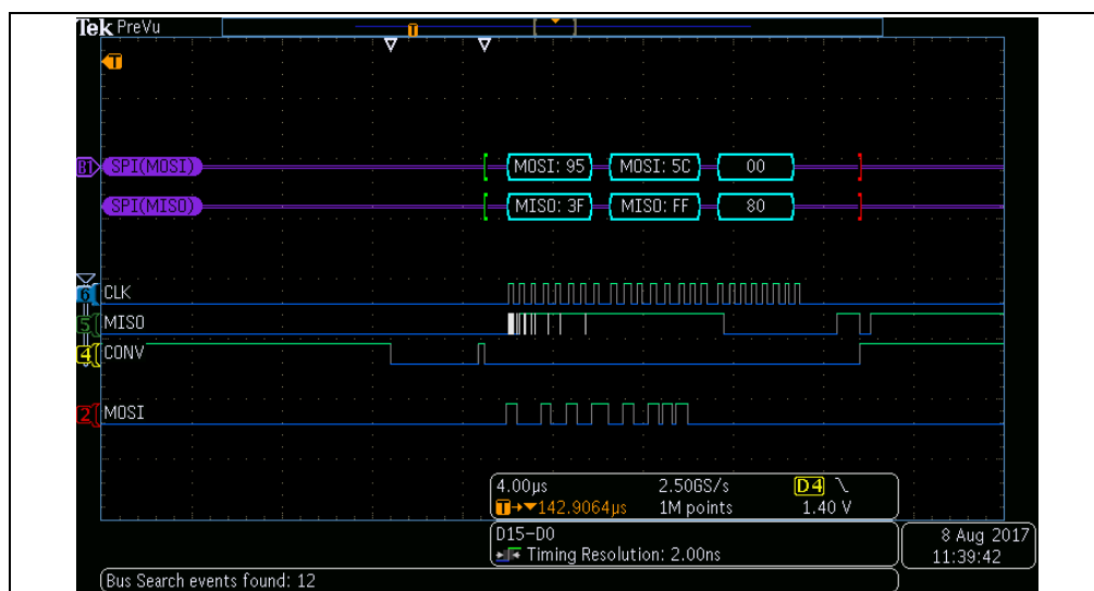
FIGURE 3-6: Read Register from ADC.
