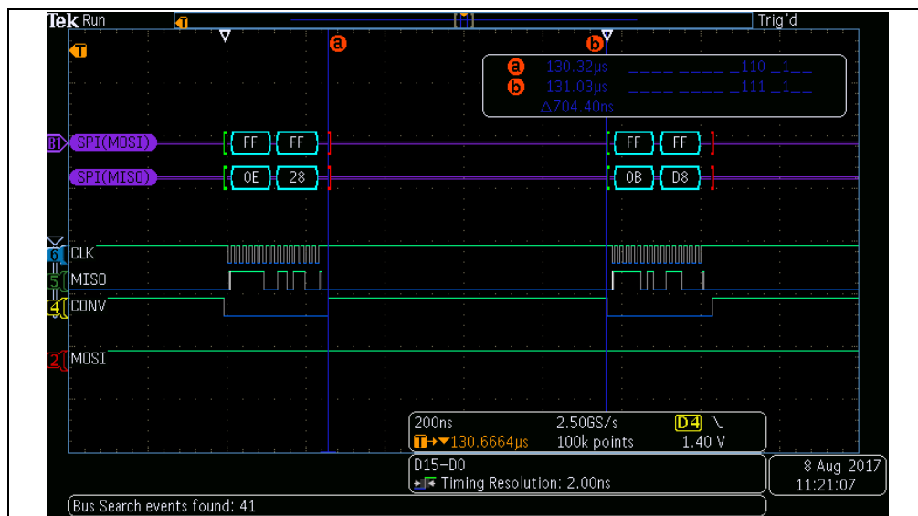
FIGURE 3-1: SPI Transfer and CONV Pulse.
