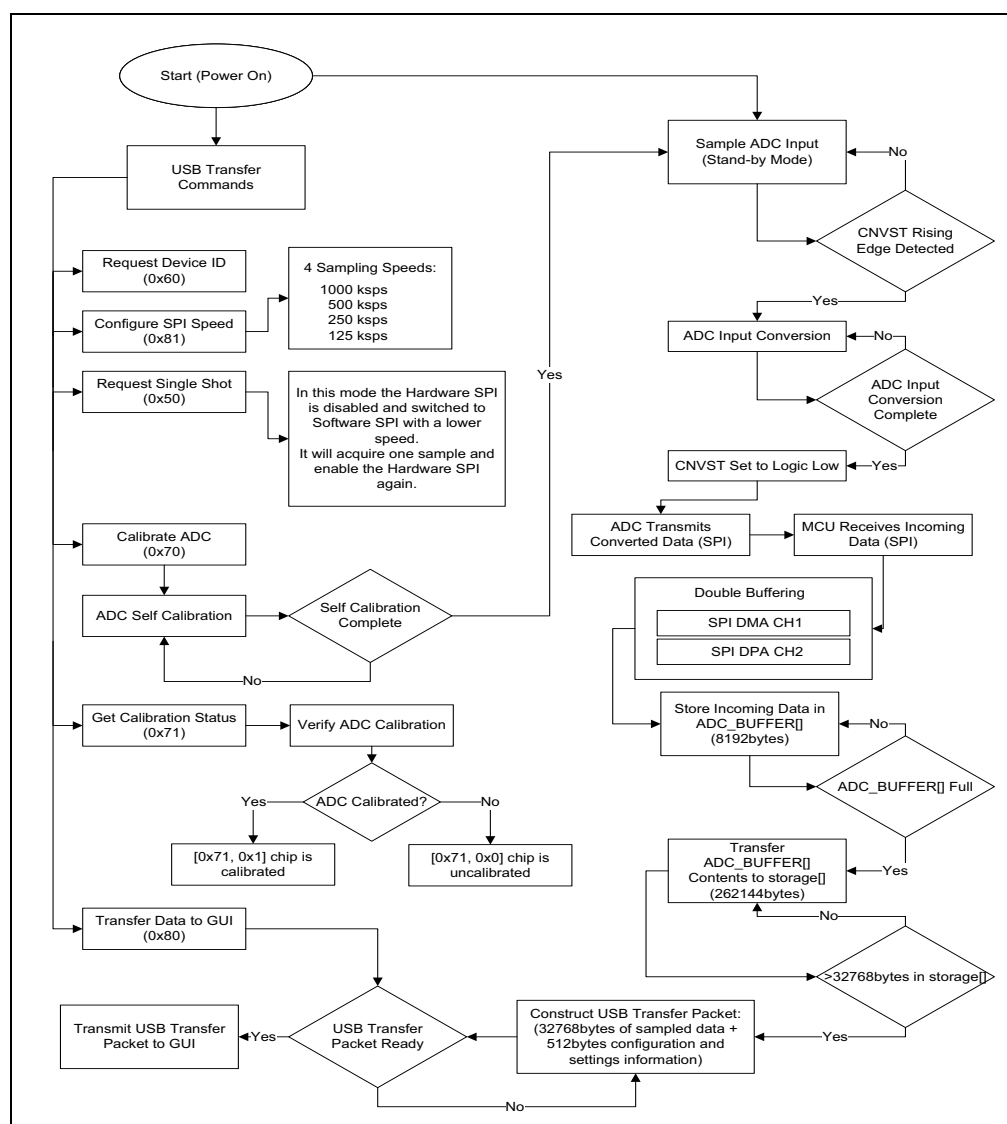
FIGURE 3-3: Firmware and ADC Samples Acquisition Flowchart.
