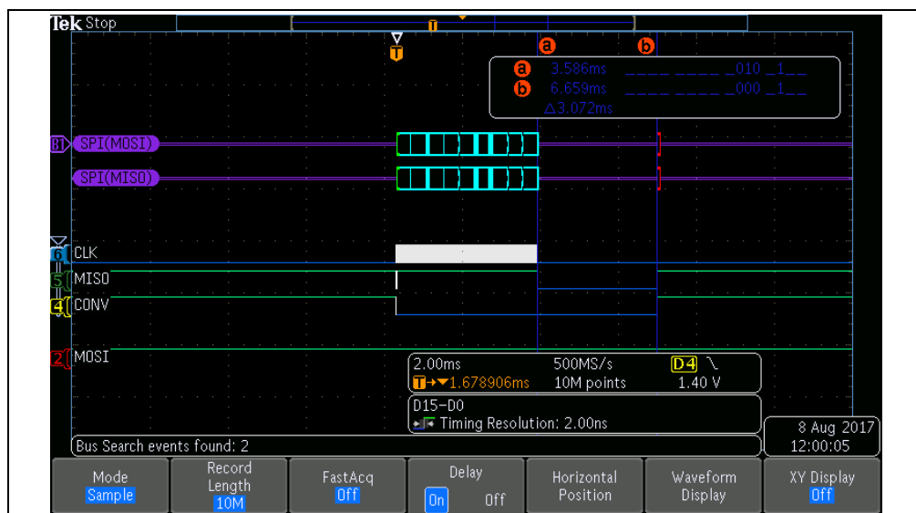
FIGURE 3-5: ADC Calibration.
