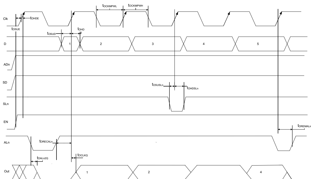
Figure 5-7. I/O Register Output Timing Diagram
