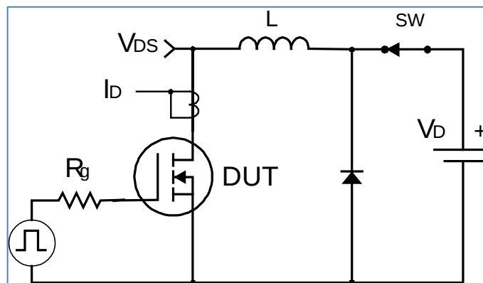
Figure 3 · UIS Test Schematic
