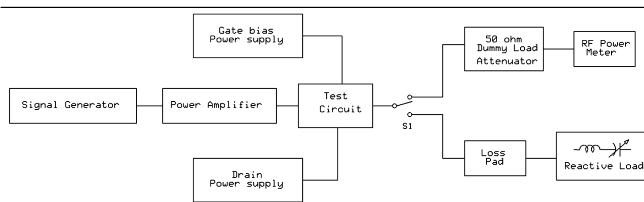
Figure 1 • VSWR Testing System
