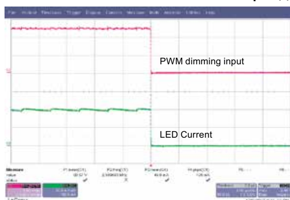
Fig. 8a: Rise time of LED Current at 40V output (5 \mu s/div)
