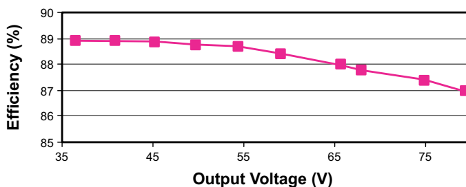
Fig. 1. Efficiency vs Output Voltage
