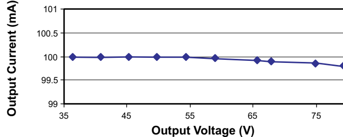
Fig. 4. Output Current vs Load Voltage
