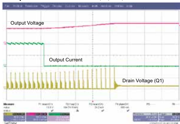
Fig. 5: Open LED Protection (20 \mu s/div)
