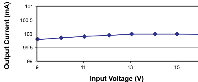
Fig. 3. Output Current vs Input Voltage
