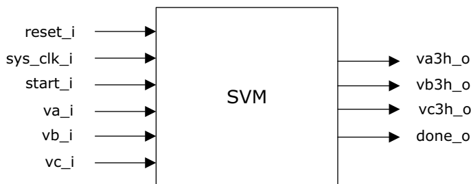
Figure 3 • SVM Hardware Block Diagram
