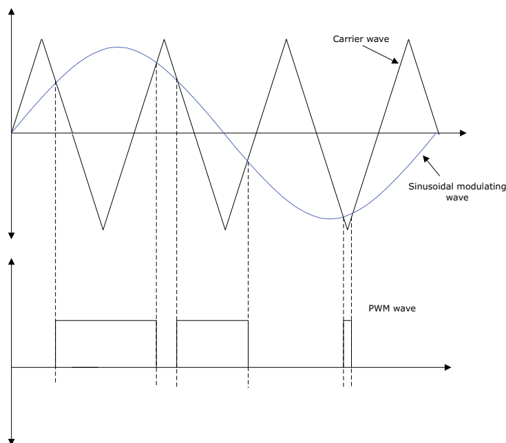
Figure 1 • Sinusoidal PWM Waveform
