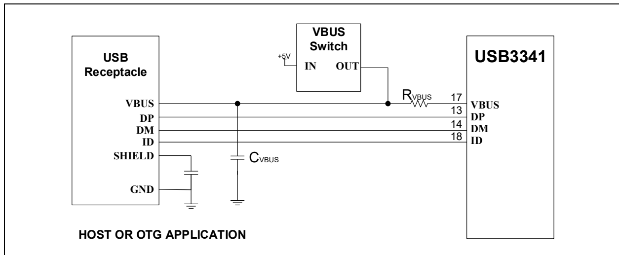
FIGURE 4-2: USB CONNECTIONS IN A HOST OR OTG APPLICATION
