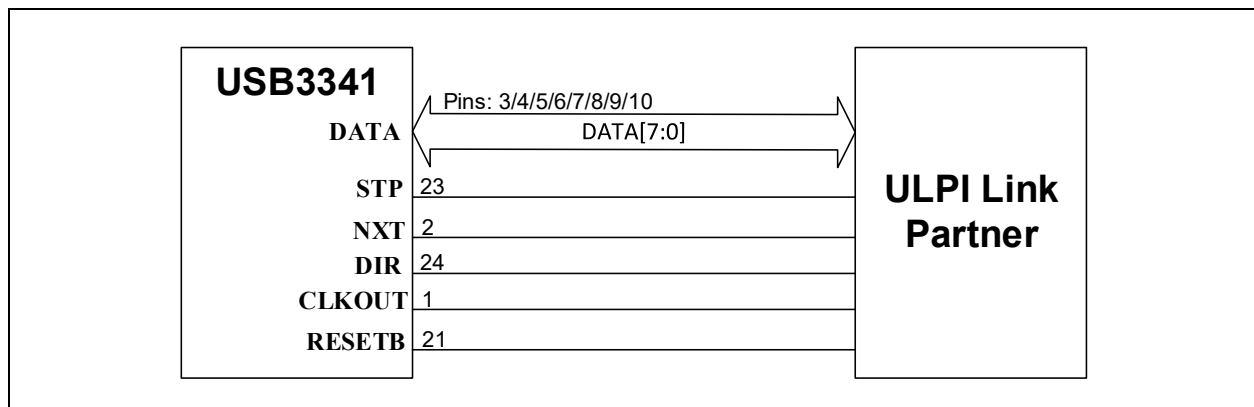
FIGURE 6-1: ULPI CONNECTIONS
