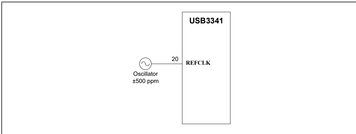
FIGURE 5-2: OSCILLATOR AND CLOCK CONNECTIONS
