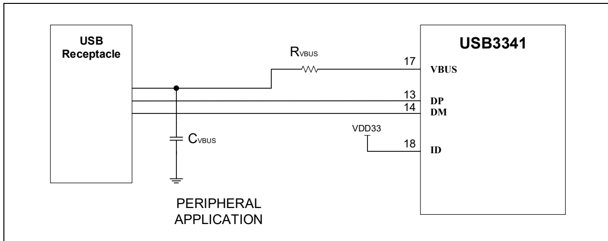
FIGURE 4-1: USB CONNECTIONS IN A PERIPHERAL APPLICATION
