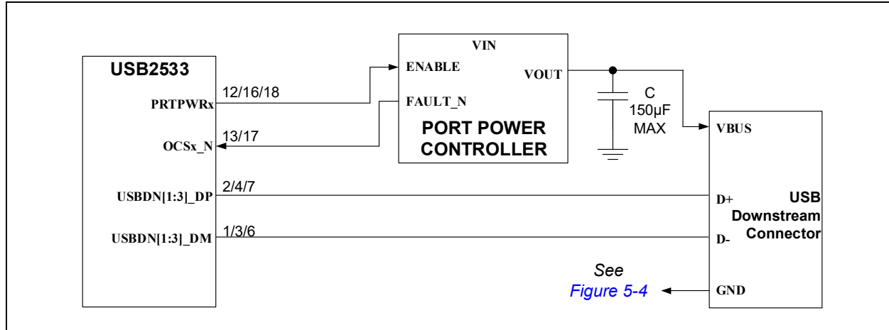
FIGURE 5-2: DOWNSTREAM VBUS AND PRTCTL1 CONNECTIONS
