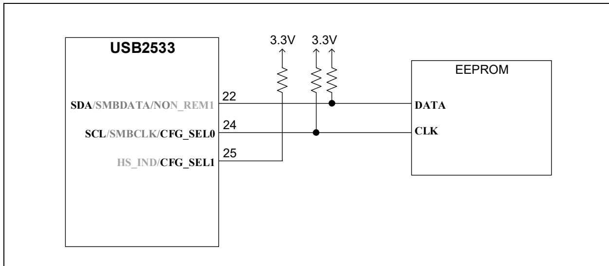
FIGURE 8-1: RECOMMENDED CONNECTIONS IF CONFIGURED VIA EEPROM
