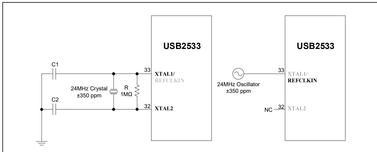
FIGURE 6-1: CRYSTAL AND OSCILLATOR CONNECTIONS
