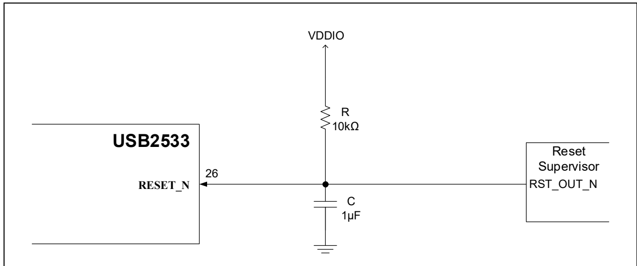
FIGURE 7-2: RESET CIRCUIT INTERFACE WITH CPU/MCU RESET OUTPUT
