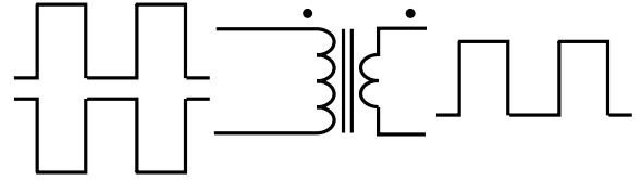
Fig. 2. Phase shifted mode for D=1 .
