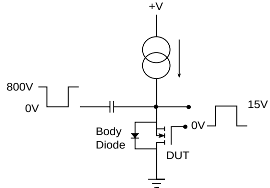
Fig. 16. Abbreviated schematic.
