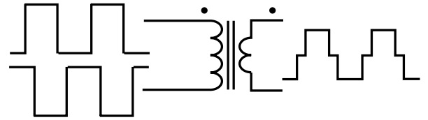
Fig. 3. Phase shifted mode for D<1
