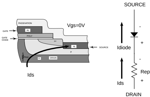
Fig. 15. Reverse current flow in the Body Diode only.
