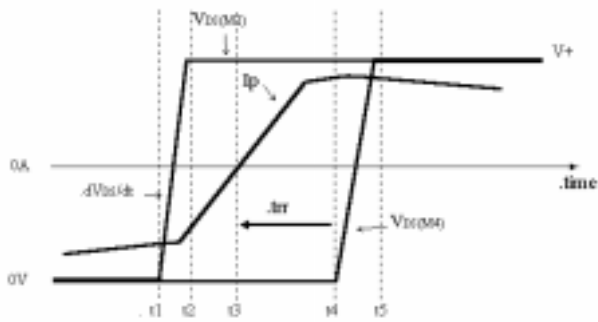
Fig. 6. Switch voltage and primary current relationship.
