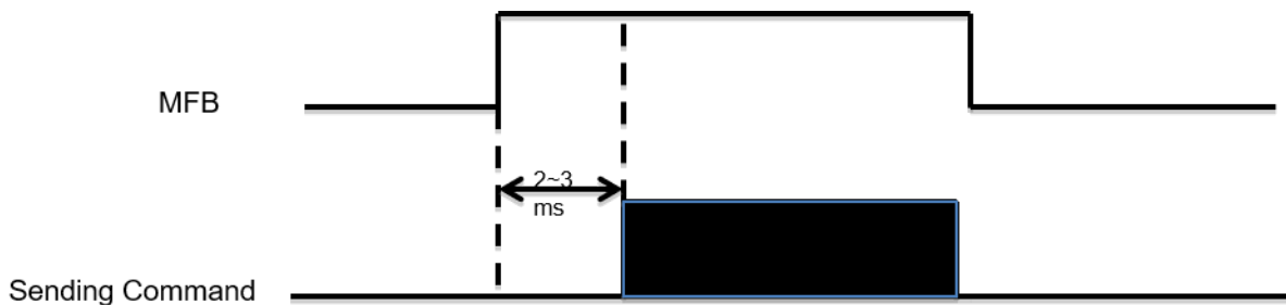
Figure 5-7. MFB Control
