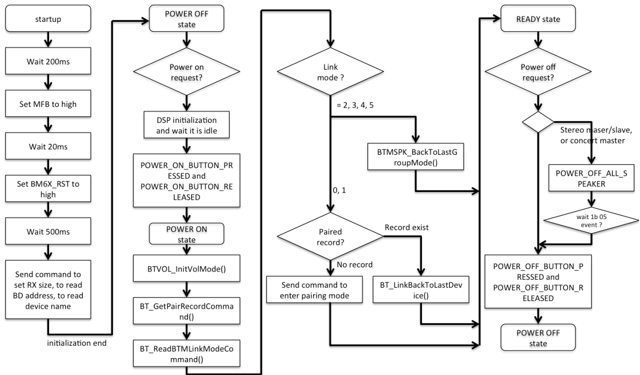
Figure 4-9. BTAPP_Task Process
