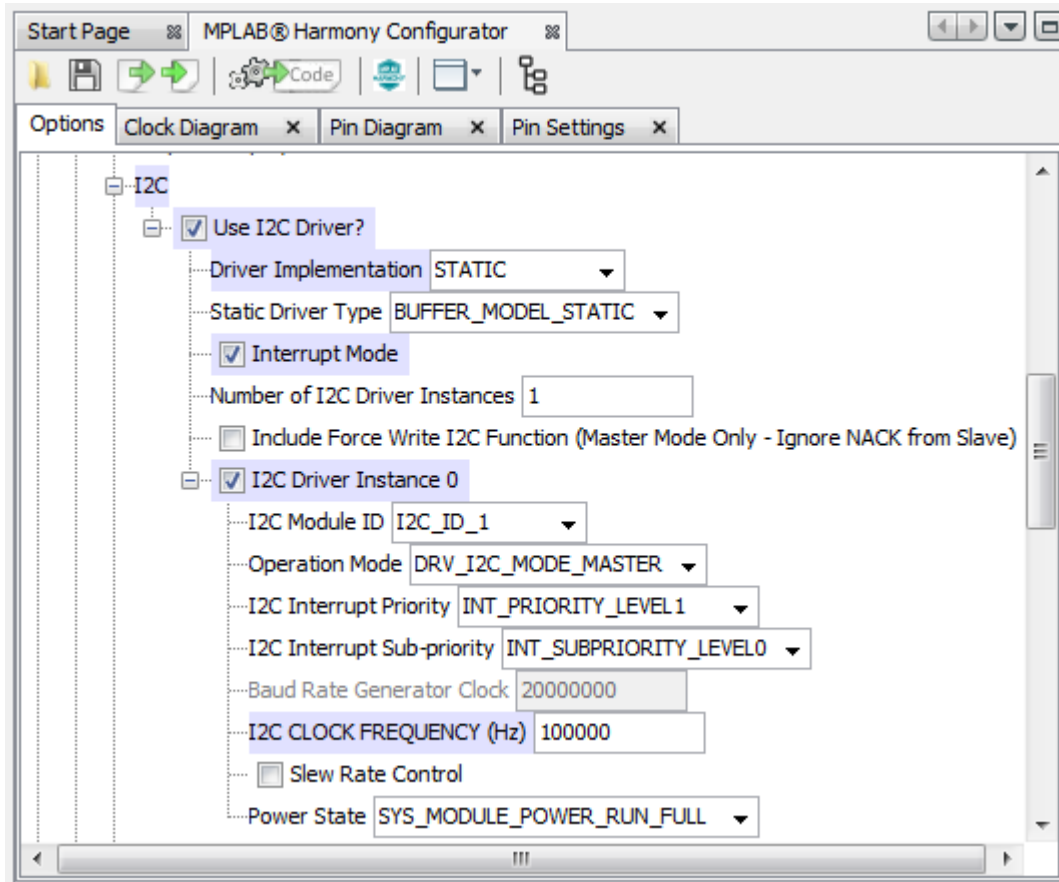
Figure 2-4. I2C Configuration
