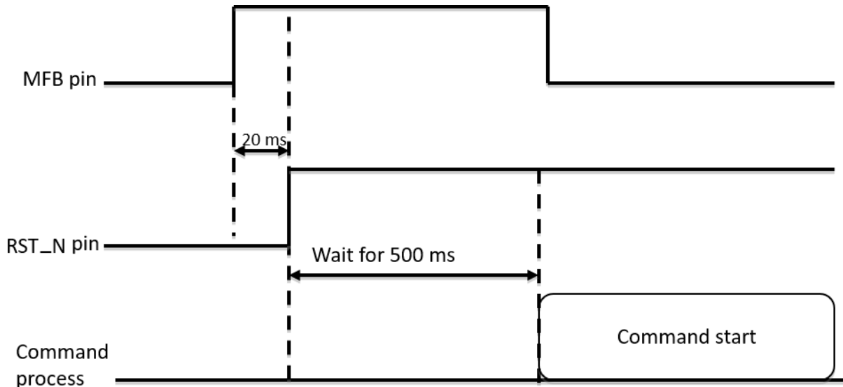
Figure 4-10. Reset Process
