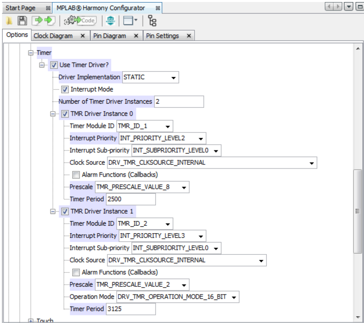
Figure 2-5. Timer Configuration
