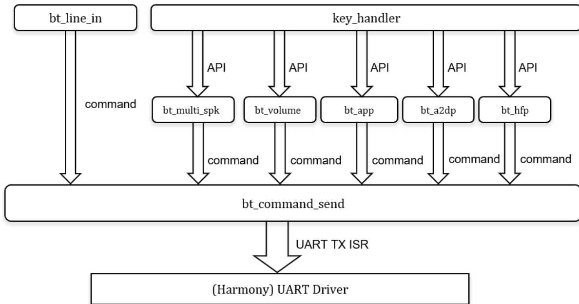
Figure 4-7. Sending Command and Command APIs
