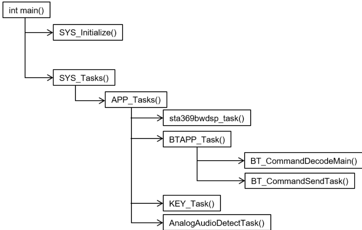
Figure 4-3. Flow Diagram
