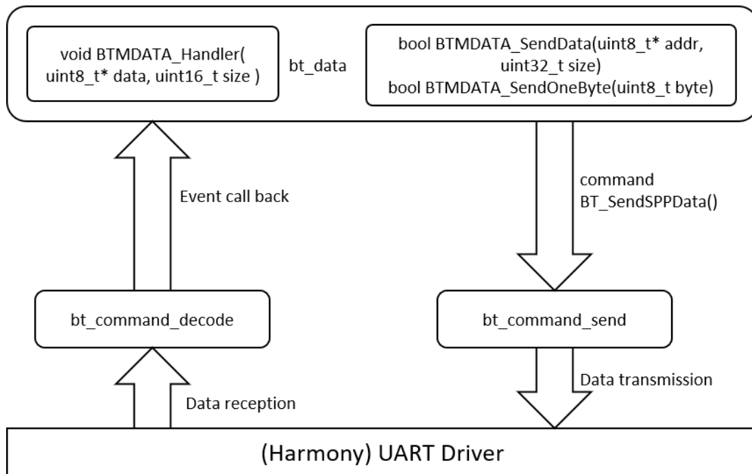
Figure 4-8. SPP/IAP/BLE Data Process
