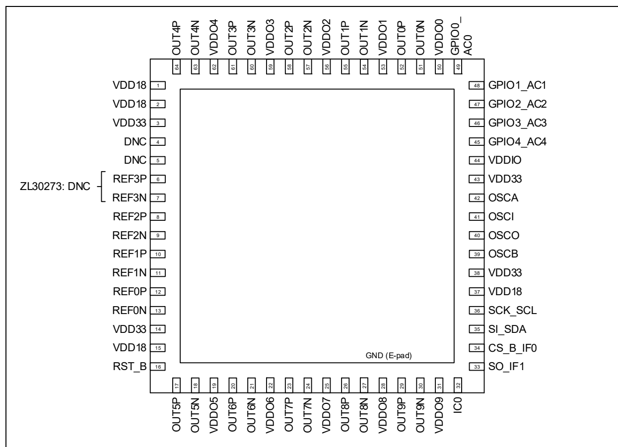
FIGURE 3-1: 64-Lead 9 mm x 9 mm VQFN (0.5 mm pitch) for ZL30273 and ZL30274.
