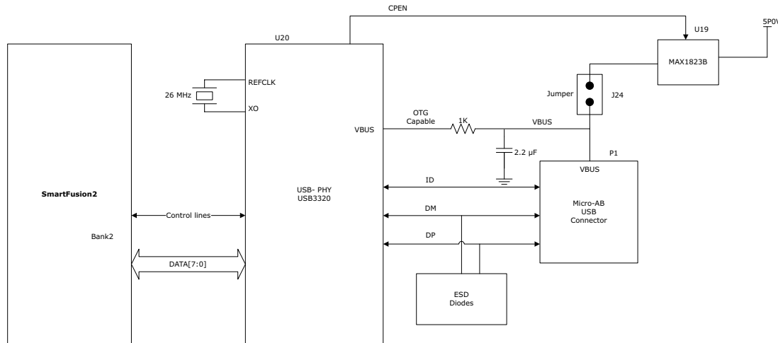
Figure 9 • USB Interface
