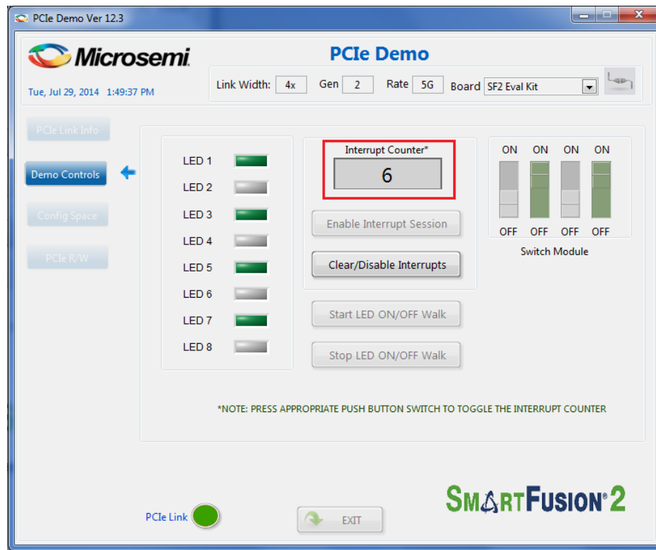
Figure 57 • Interrupt Counter
