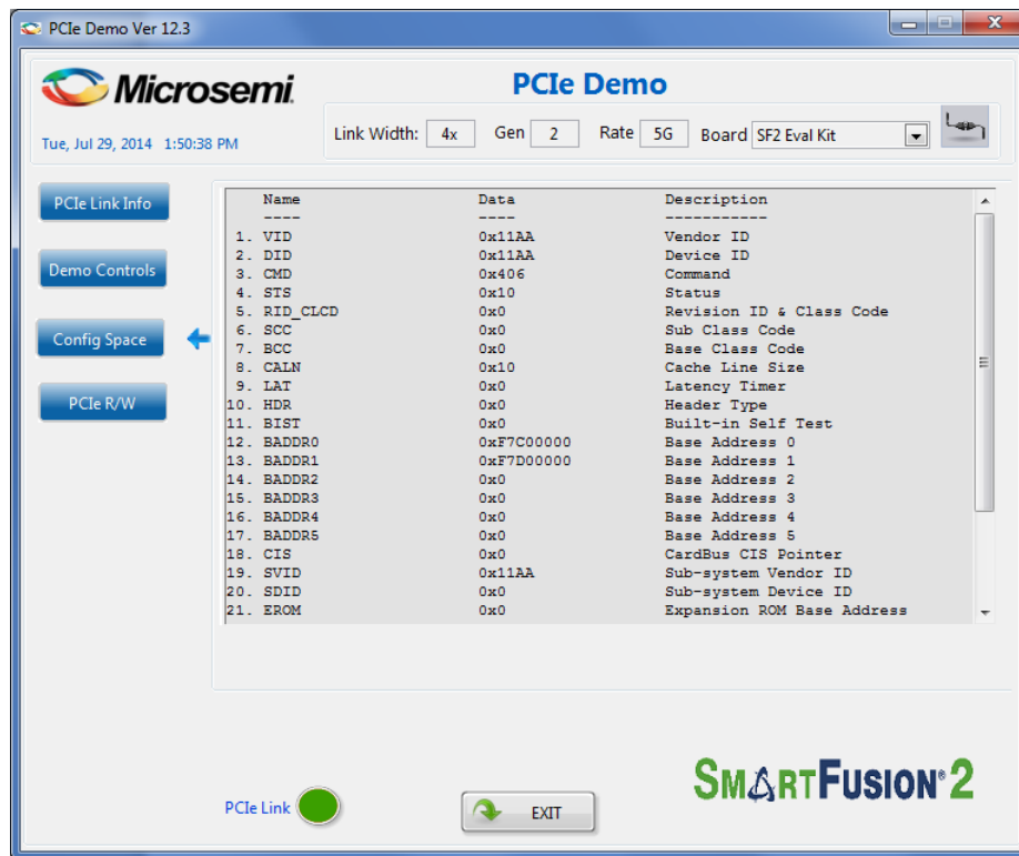
Figure 58 • Configuration Space
