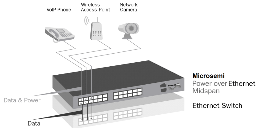
Figure 4-1. Typical Installation
