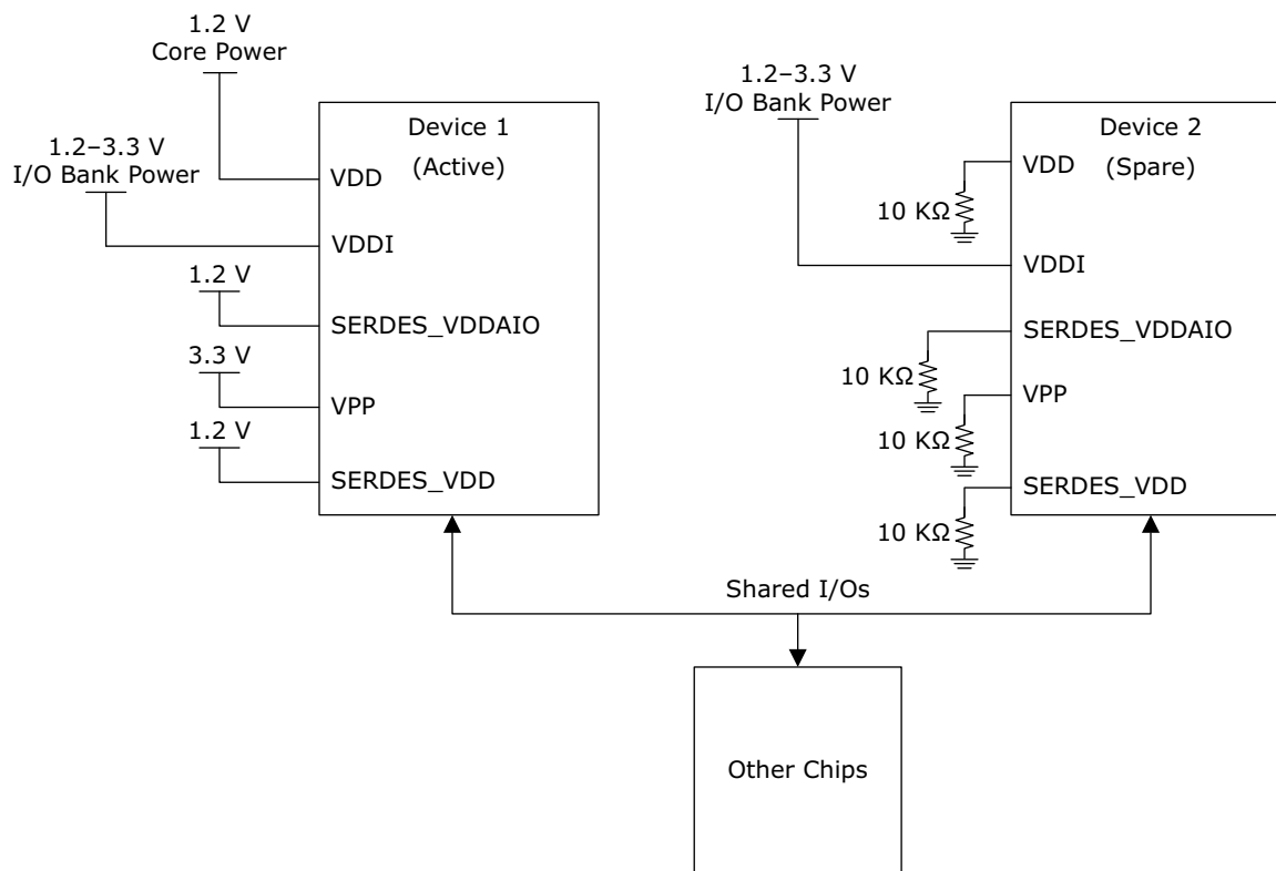
Figure 4 • Cold Sparing
