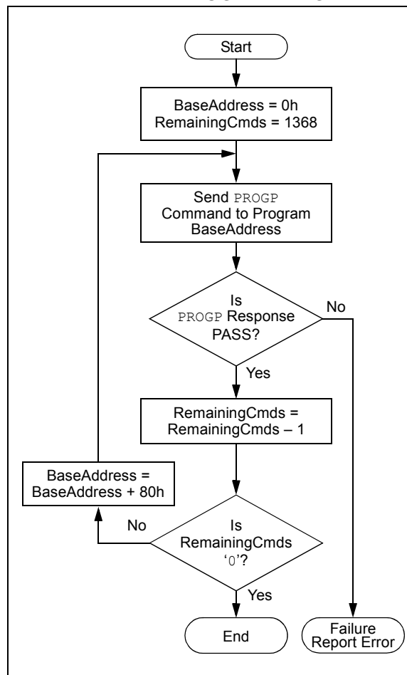
FIGURE 4-5: FLOWCHART FOR MULTIPLE WORD PROGRAMMING
