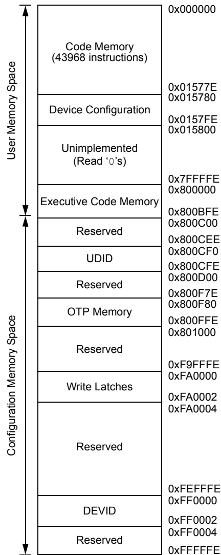
FIGURE 2-9: PROGRAM MEMORY MAP FOR dsPIC33EV128GM00X/10X DEVICES (1)
