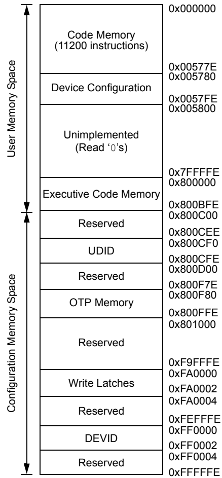
FIGURE 2-7: PROGRAM MEMORY MAP FOR dsPIC33EV32GM00X/10X DEVICES (1)
