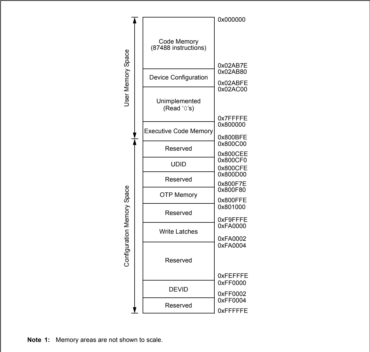
FIGURE 2-10: PROGRAM MEMORY MAP FOR dsPIC33EV256GM00X/10X DEVICES (1)
