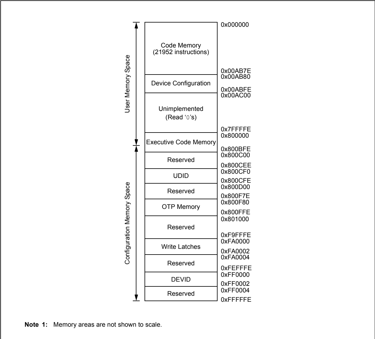
FIGURE 2-8: PROGRAM MEMORY MAP FOR dsPIC33EV64GM00X/10X DEVICES (1)
