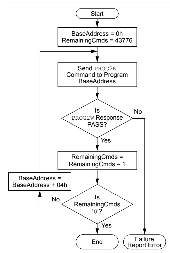
FIGURE 4-4: FLOWCHART FOR DOUBLE-WORD PROGRAMMING
