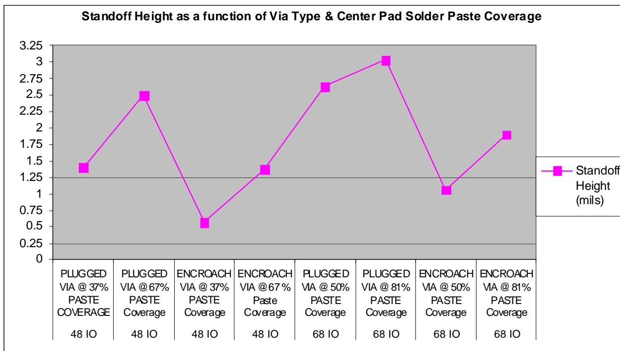
Figure 6. Standoff height as a function of via type and paste coverage
