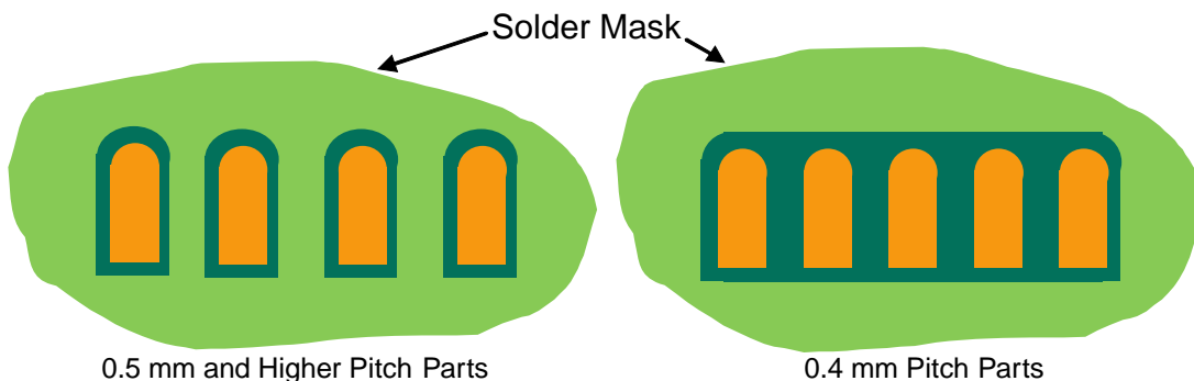
Figure 2. Solder mask definition for perimeter lands
