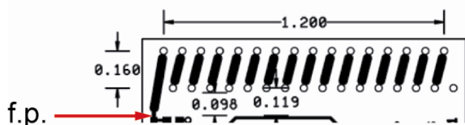
Fig. 5 – Dimensions on the top layer (inches)
