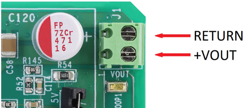
Figure 2-2. V out Connectors
