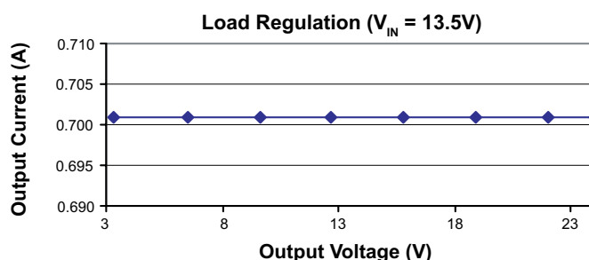
Fig.3 Output Current vs. Output Voltage
