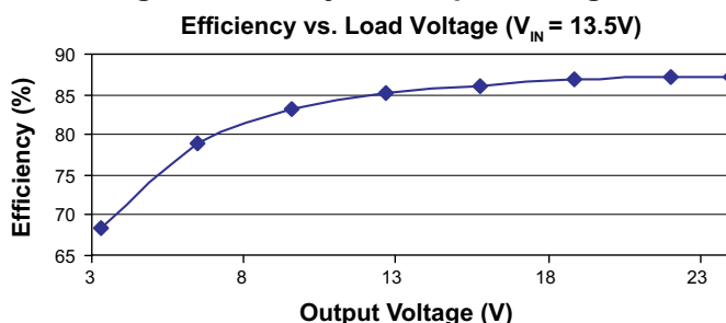
Fig.1 Efficiency vs. Output Voltage
