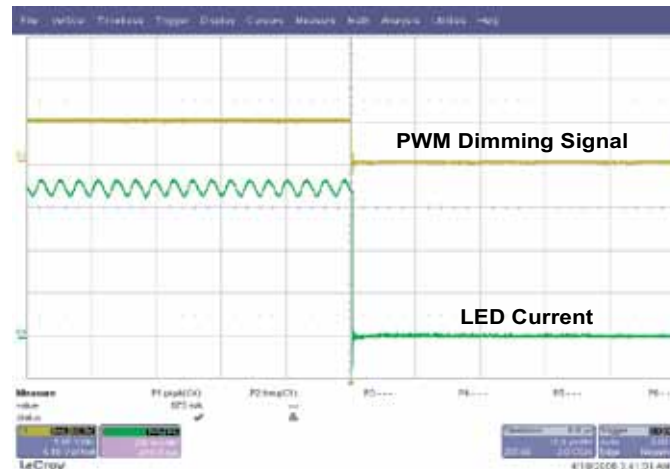
Fig.9b. Fall Time (10µs/div)
