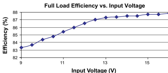
Fig.2 Efficiency vs. Input Voltage
