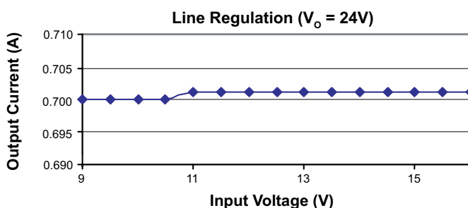
Fig.4 Output Current vs. Input Voltage
