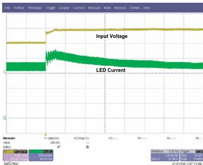
Fig. 10. Response of the HV9911DB4 to an input voltage change (Time Scale: 1ms/div)
