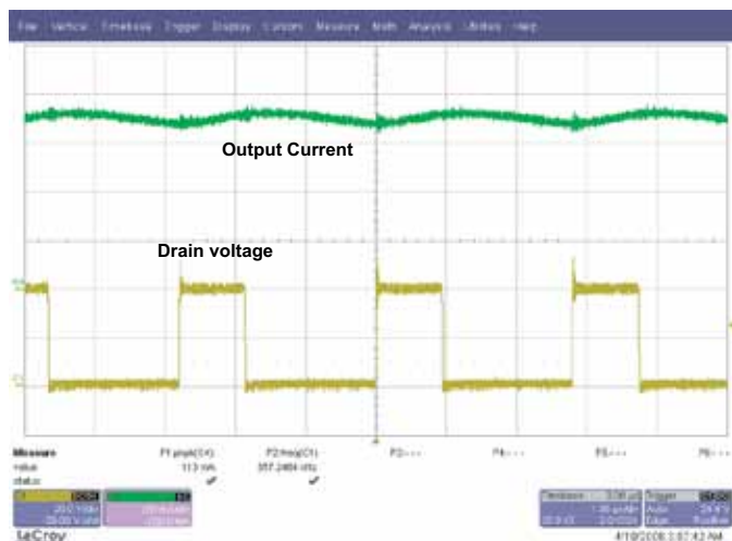
Fig.5. Switching waveforms for the HV9911DB4
