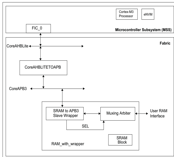
Figure 4 • Design Example Block Diagram
