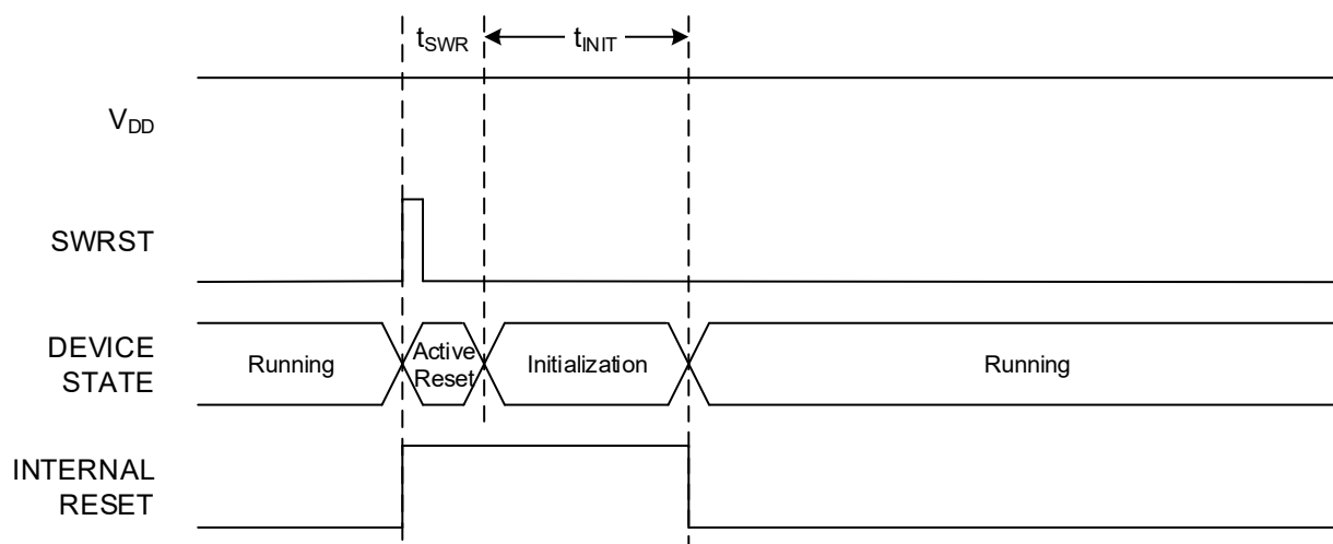
Figure 14-6. Software Reset
