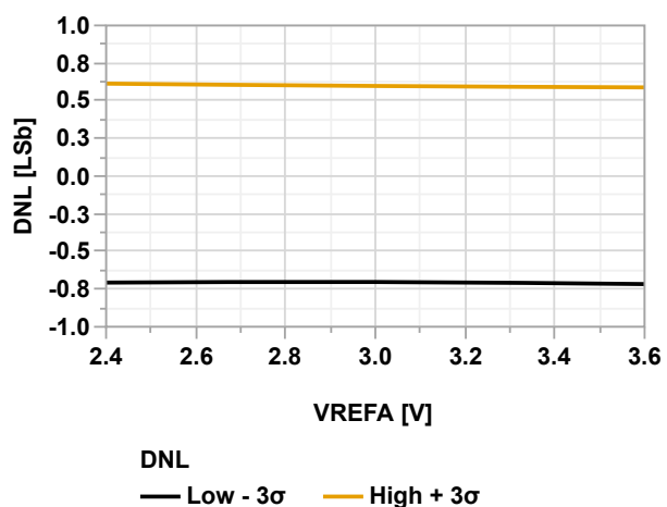
Figure 39-127. DNL vs. V_{\text{REFA}} (ADC Differential Mode @60 kps, V_{\text{DD}} = 3.6\text{V} , T = 25^\circ\text{C} )
