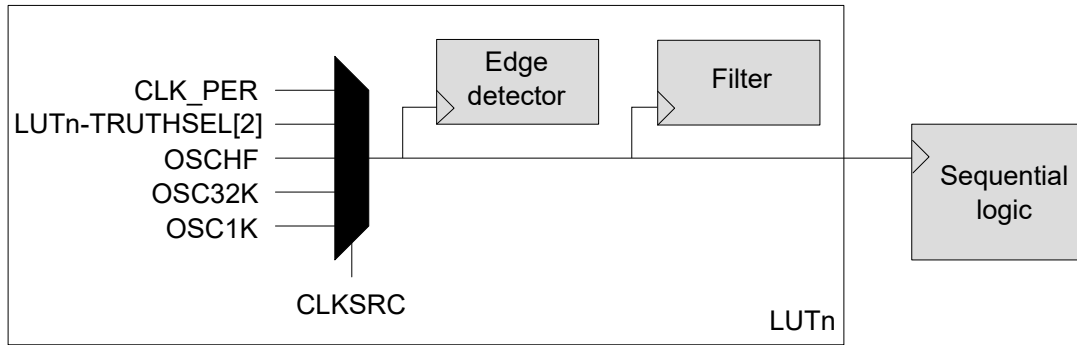
Figure 31-11. Clock Source Settings
