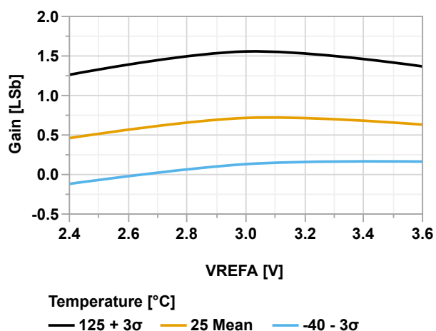
Figure 39-122. Negative Gain Error vs. V_{\text{REFA}} (ADC Differential Mode @60 kps, V_{\text{DD}} = 3.6\text{V} )
