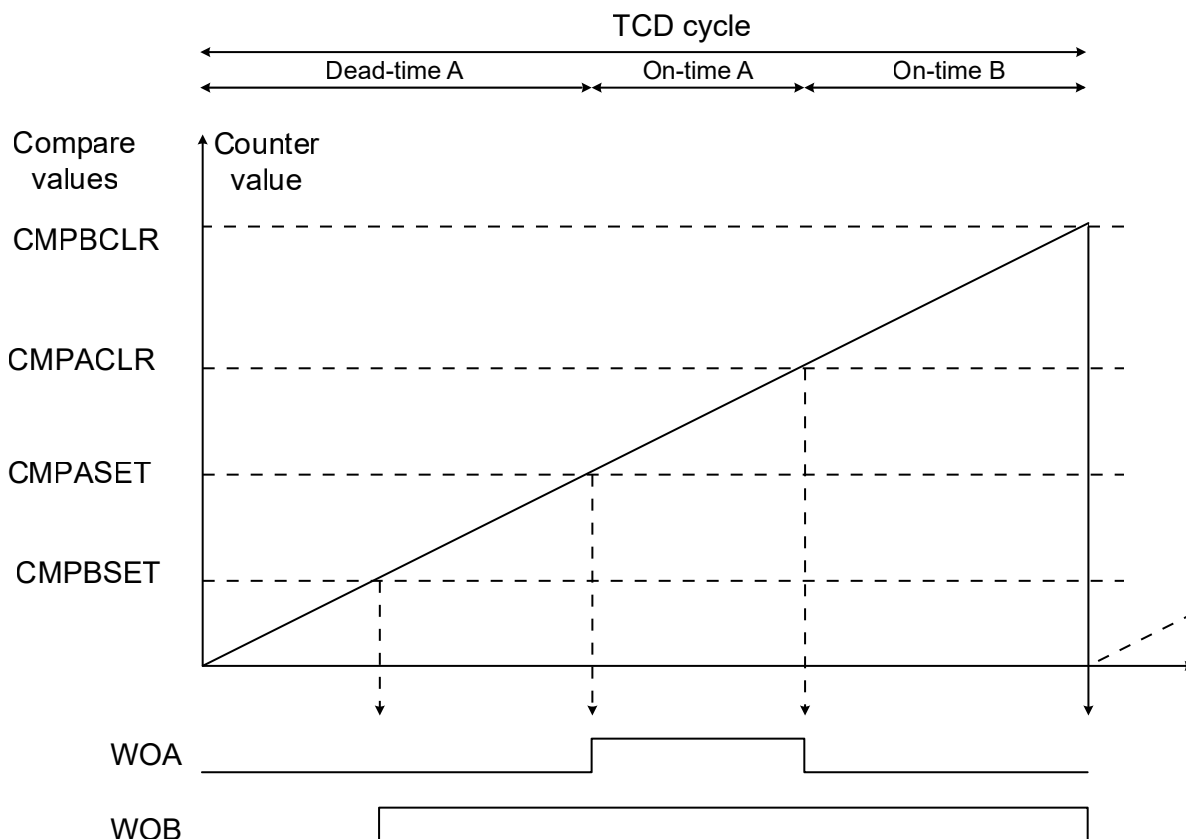
Figure 25-4. One Ramp Mode with CMPBSET < CMPASET
