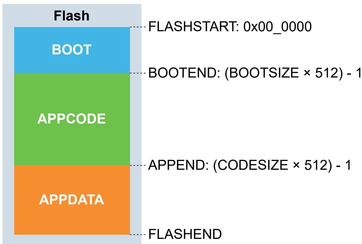
Figure 11-2. Flash Sections Sizes and Locations
