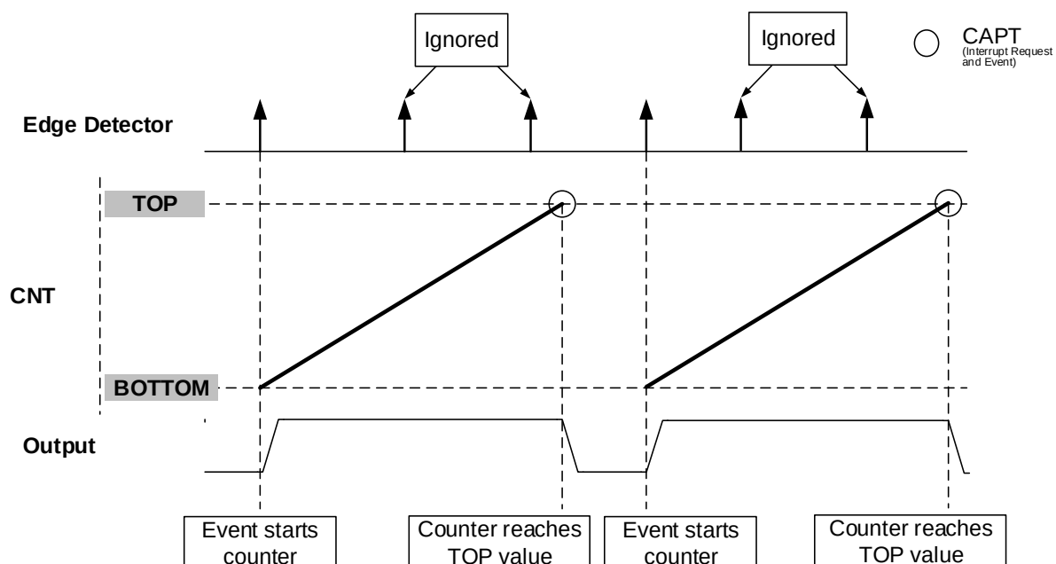
Figure 24-9. Single-Shot Mode
