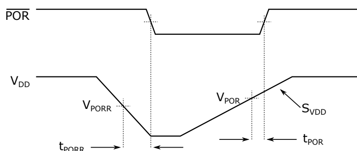
Figure 38-1. \overline{POR} and \overline{PORR} with Slow Rising V_{DD}
