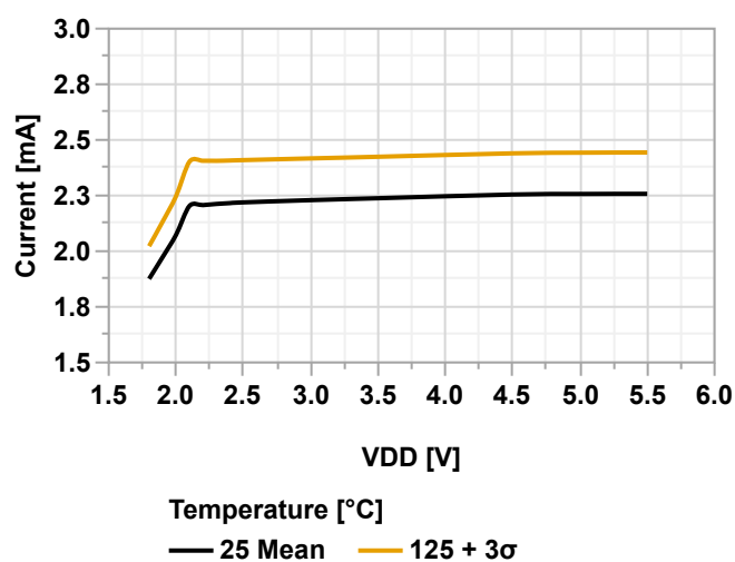
Figure 39-9. Idle Power Consumption vs. V_{DD} (MCLKCTRLA.CLKSEL = OSCHF, OSCHF = 24 MHz)
