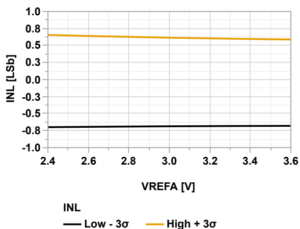
Figure 39-131. INL vs. V_{\text{REFA}} (ADC Differential Mode @60 kps, V_{\text{DD}} = 3.6\text{V} , T = 25^\circ\text{C} )
