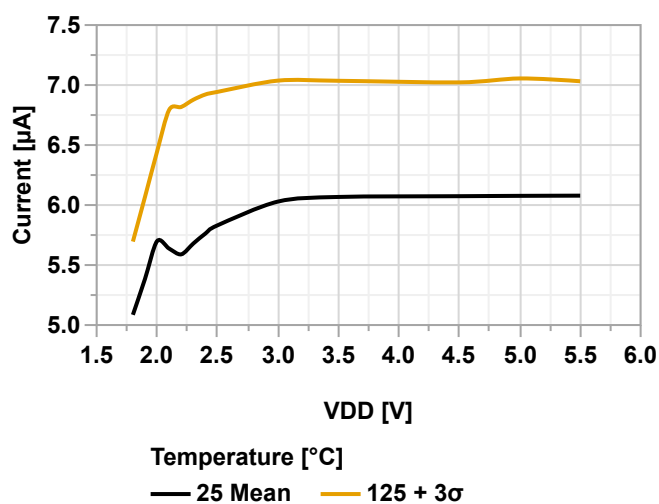
Figure 39-36. TWI Power Consumption vs. V_{DD} (TWI Client Mode @100 kHz)
