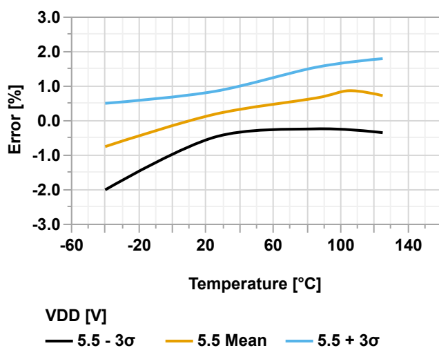
Figure 39-93. ADC0REF Voltage Error vs. Temperature ( V_{DD} = 5.5V , V_{VREF} = 2.5V )
