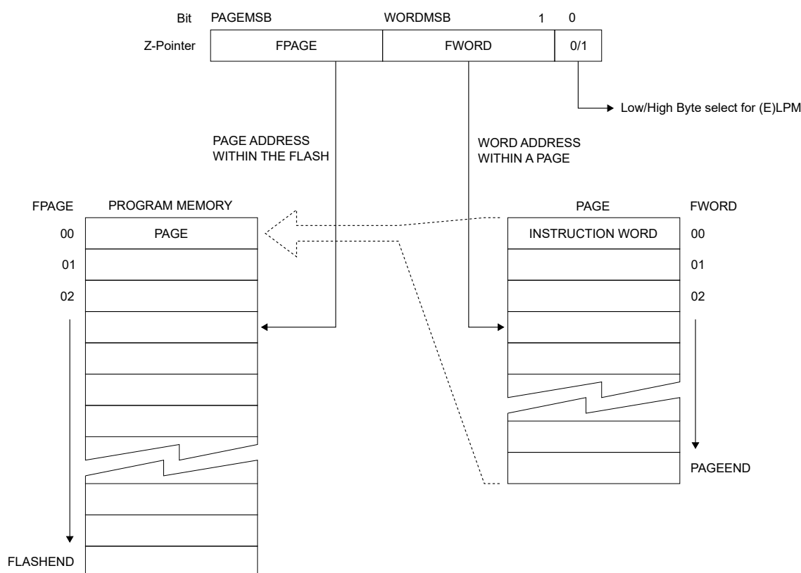
Figure 11-3. Flash Addressing for Self-Programming
