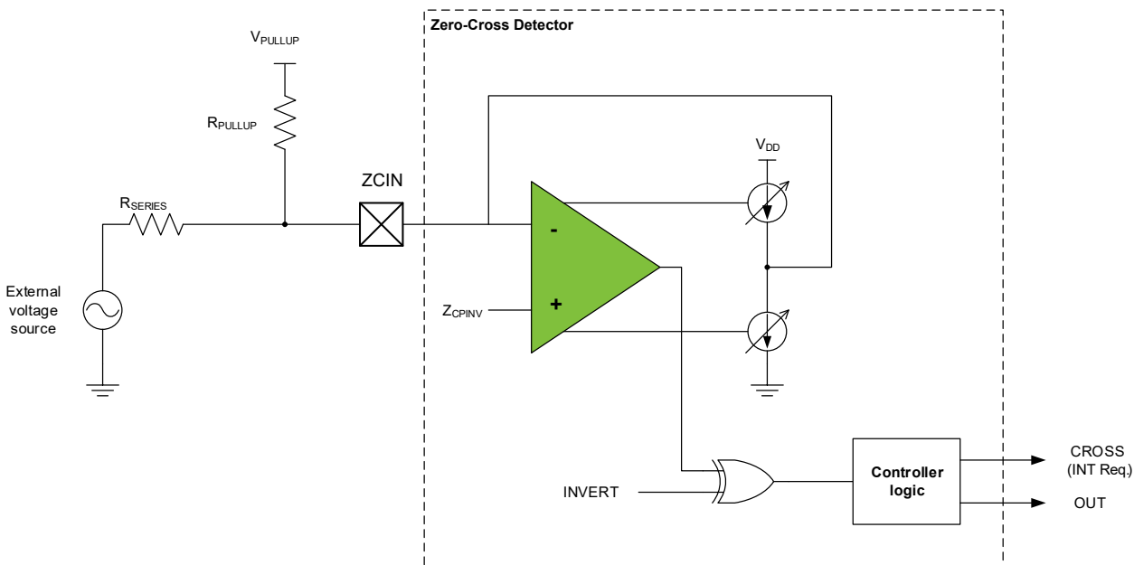
Figure 35-5. External Voltage Source Referenced to Ground
