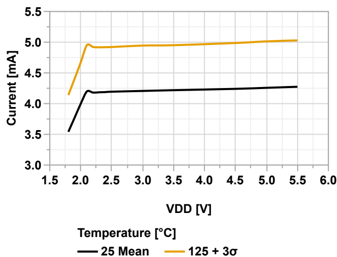
Figure 39-2. Active Power Consumption vs. V_{DD} (MCLKCTRLA.CLKSEL = EXTCLK, EXTCLK = 24 MHz)
