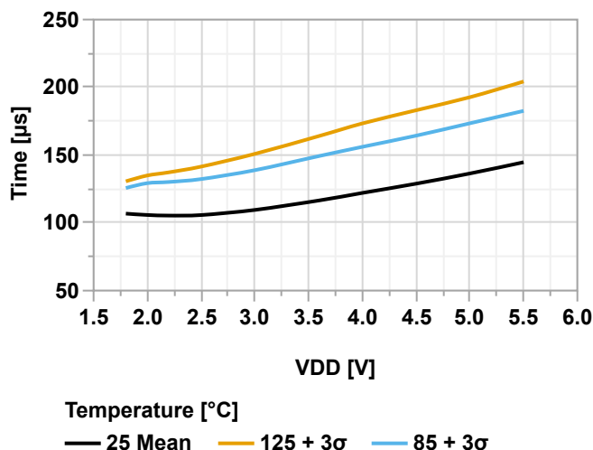
Figure 39-46. Wake-up Time from Power-Down vs. V_{DD} (OSCHF = 4 MHz, VREGCTRL = AUTO)
