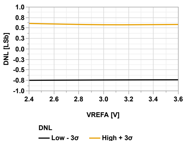
Figure 39-126. DNL vs. V_{\text{REFA}} (ADC Differential Mode @60 kps, V_{\text{DD}} = 3.6\text{V} , T = -40^\circ\text{C} )
