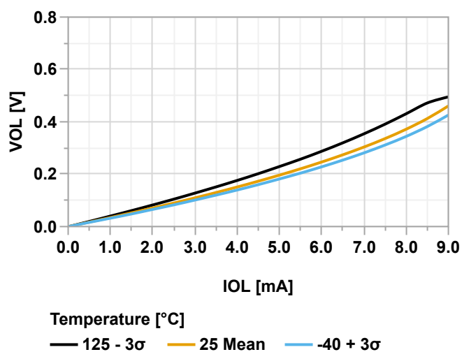
Figure 39-82. Output Pin - Maximum V_{OL} vs. Current, V_{DD} = 1.8V
