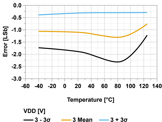
Figure 39-149. Offset Error vs. Temperature ( V_{\text{REFA}} = V_{\text{DD}} = 3.0\text{V} )
