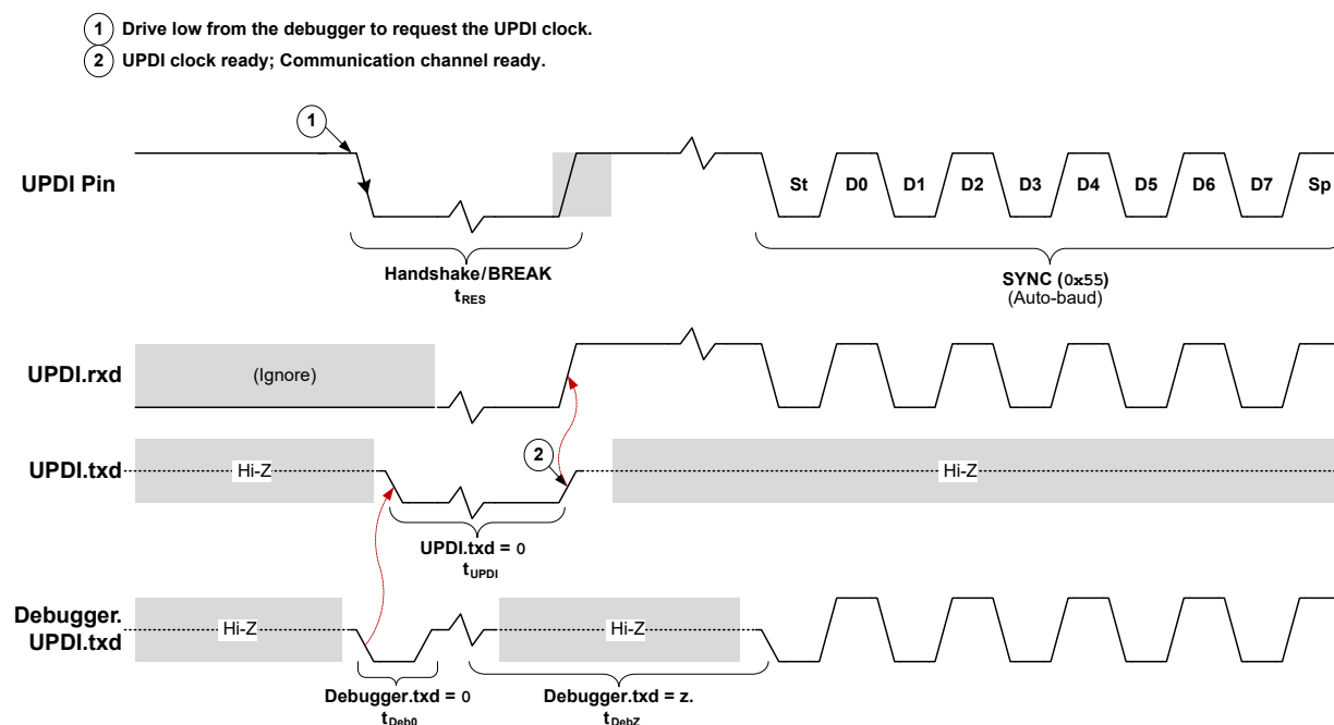
Figure 38-8. UPDI Enable Sequence with Dedicated UPDI Pin
