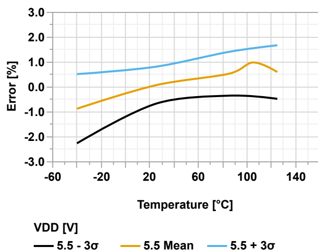
Figure 39-95. ADC0REF Voltage Error vs. Temperature ( V_{DD} = 5.5V , V_{VREF} = 4.096V )
