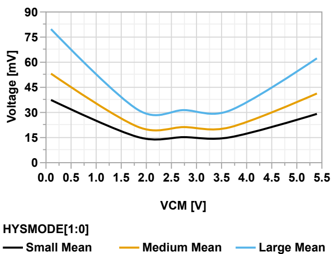
Figure 39-146. Input Hysteresis vs. Common Mode Voltage ( V_{DD} = 5.5V )
