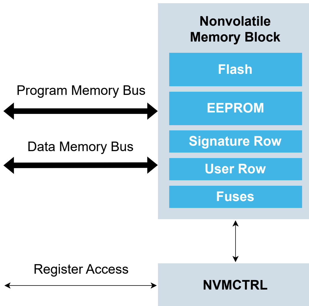
Figure 11-1. NVMCTRL Block Diagram
