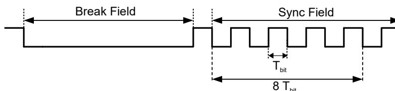
Figure 27-9. Auto-Baud Timing
