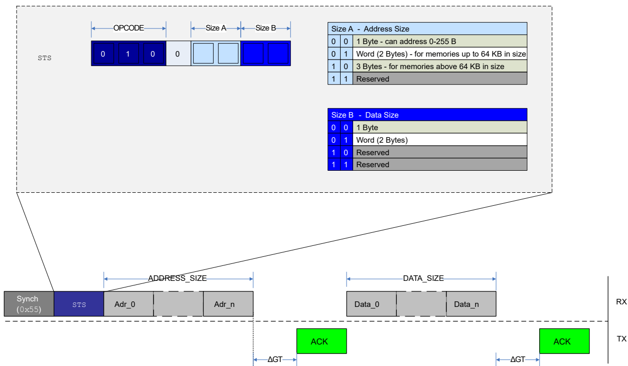
Figure 36-10. STS Instruction Operation
