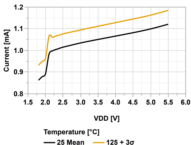
Figure 39-20. ADC Power Consumption vs. V_{DD} (ADC @120 ksp/s)
