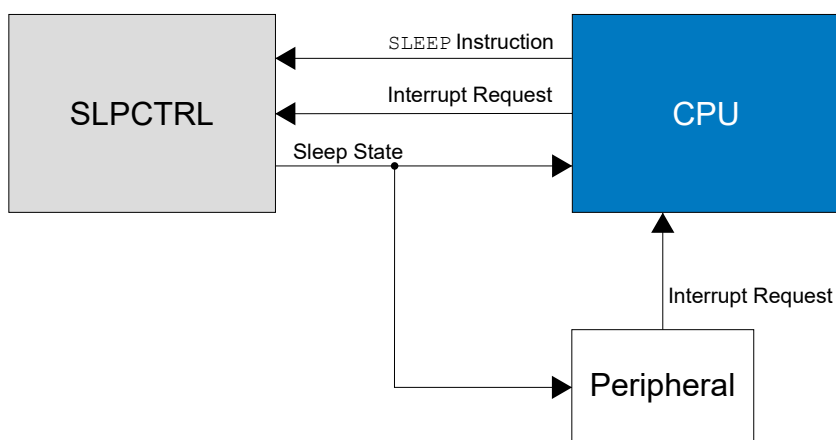
Figure 13-1. SLPCTRL Block Diagram
