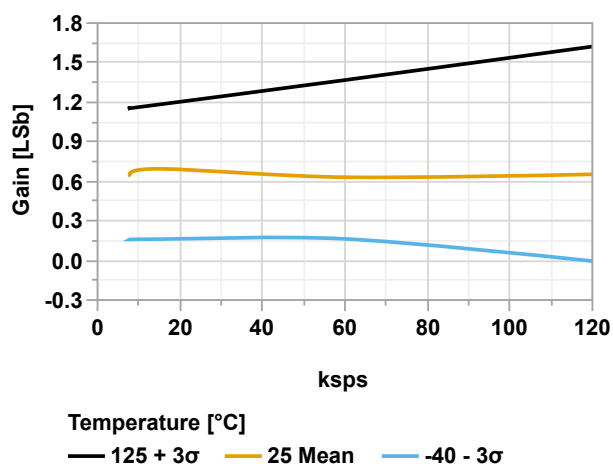
Figure 39-123. Negative Gain Error vs. Sample Rate (ADC Differential Mode, V_{\text{REFA}} = V_{\text{DD}} = 3.6\text{V} )
