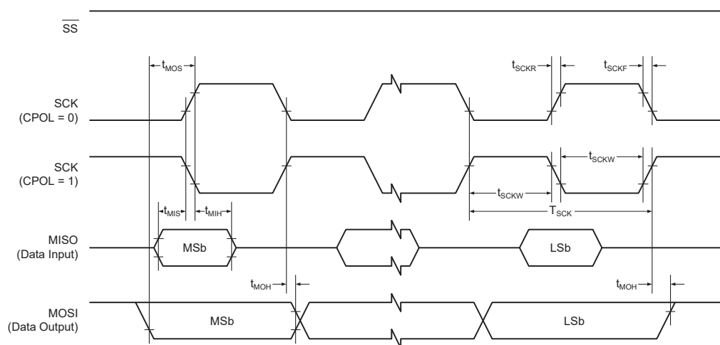
Figure 38-4. USART in SPI Mode - Timing Requirements in Host Mode
