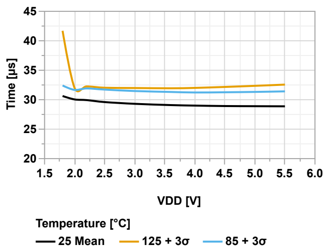
Figure 39-47. Wake-up Time from Power-Down vs. V_{DD} (OSCHF = 4 MHz, VREGCTRL = FULL)
