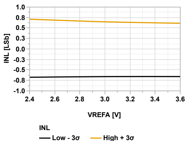
Figure 39-130. INL vs. V_{\text{REFA}} (ADC Differential Mode @60 kps, V_{\text{DD}} = 3.6\text{V} , T = -40^\circ\text{C} )
