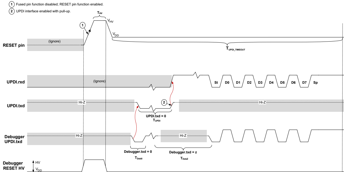
Figure 38-9. UPDI Enable Sequence by High-Voltage (HV) Programming
