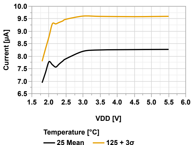
Figure 39-37. USART Power Consumption vs. V_{DD} (USART Enabled @9600 Baud)
