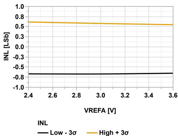
Figure 39-132. INL vs. V_{\text{REFA}} (ADC Differential Mode @60 kps, V_{\text{DD}} = 3.6\text{V} , T = 85^\circ\text{C} )
