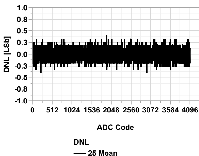
Figure 39-114. DNL vs. ADC code (ADC Single Ended Mode @60 kps, V_{\text{DD}} = 3.0\text{V} )
