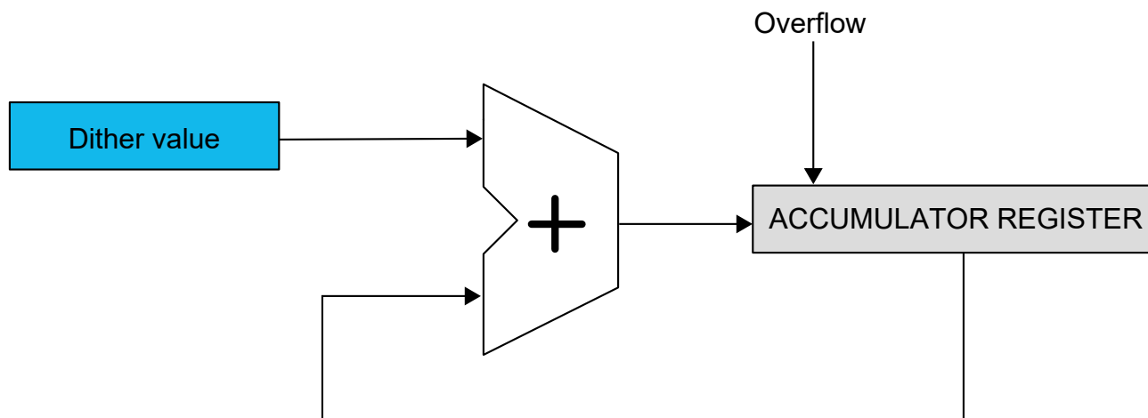
Figure 25-27. Dither Logic
