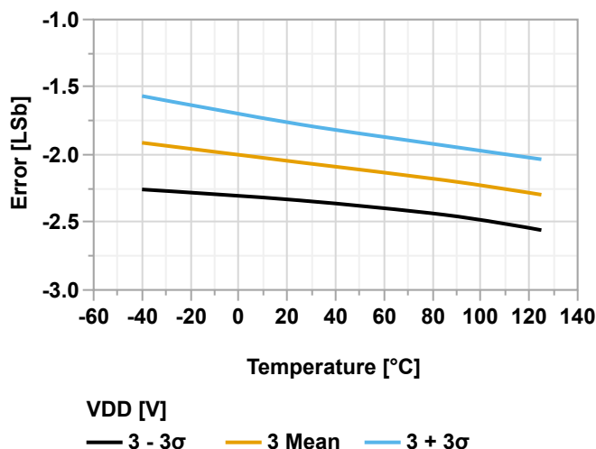
Figure 39-157. Offset Error vs. Temperature ( V_{\text{REFA}} = V_{\text{DD}} = 3.0\text{V} )
