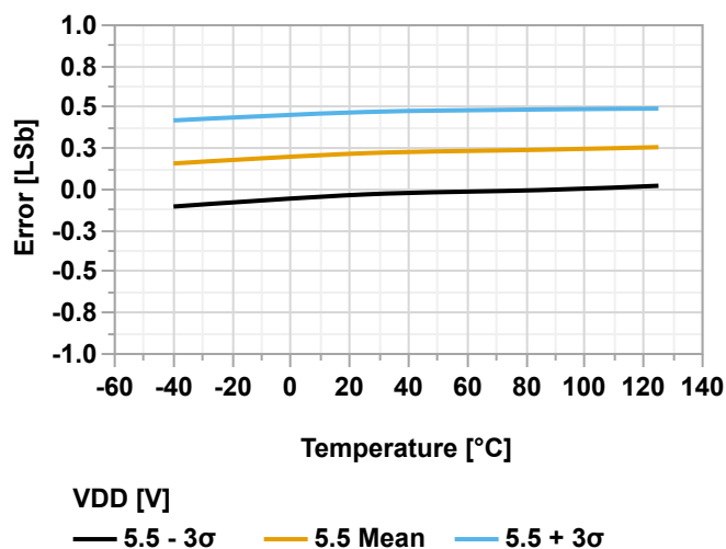
Figure 39-158. Offset Error vs. Temperature ( V_{\text{REFA}} = V_{\text{DD}} = 5.5\text{V} )
