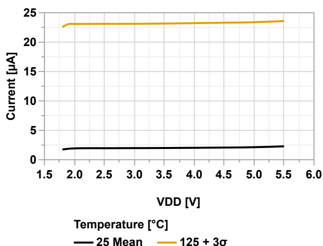
Figure 39-13. Standby Power Consumption vs. V_{DD} (RTC.CLKSEL = XOSC32K, XOSC32KCTRLA.LPMODE = 1)
