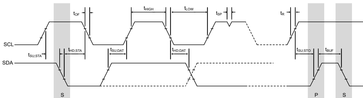
Figure 38-7. TWI - Timing Requirements
