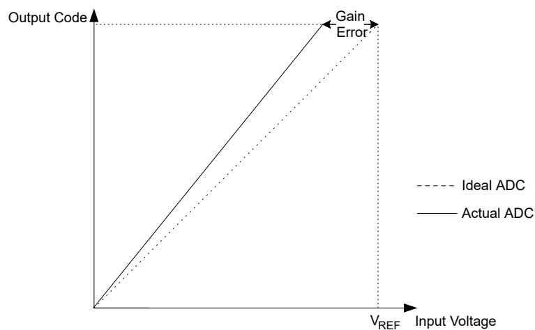
Figure 6-2. Gain Error
