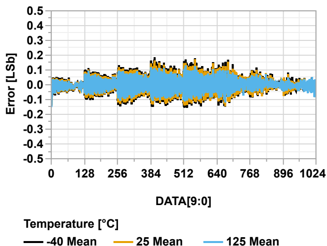
Figure 39-153. INL vs. DAC Code ( V_{\text{REFA}} = V_{\text{DD}} = 3.0\text{V} )
