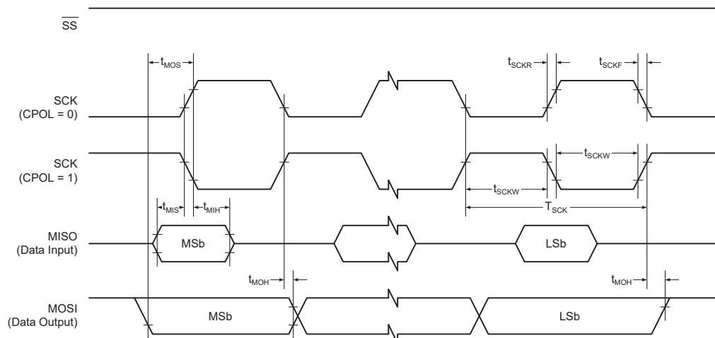
Figure 38-5. SPI - Timing Requirements in Host Mode
