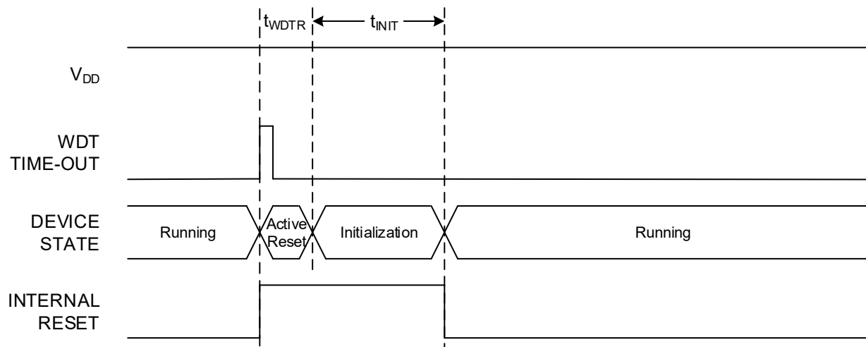
Figure 14-5. Watchdog Reset
