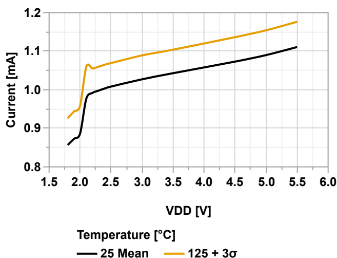
Figure 39-19. ADC Power Consumption vs. V_{DD} (ADC @60 ksp/s)
