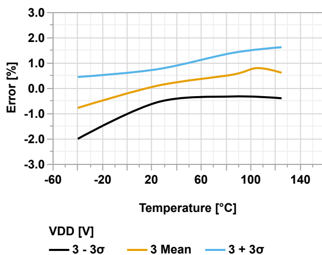
Figure 39-94. ADC0REF Voltage Error vs. Temperature ( V_{DD} = 3.0V , V_{VREF} = 2.5V )
