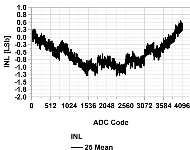
Figure 39-115. INL vs. ADC code (ADC Single Ended Mode @60 kps, V_{\text{DD}} = 3.0\text{V} )
